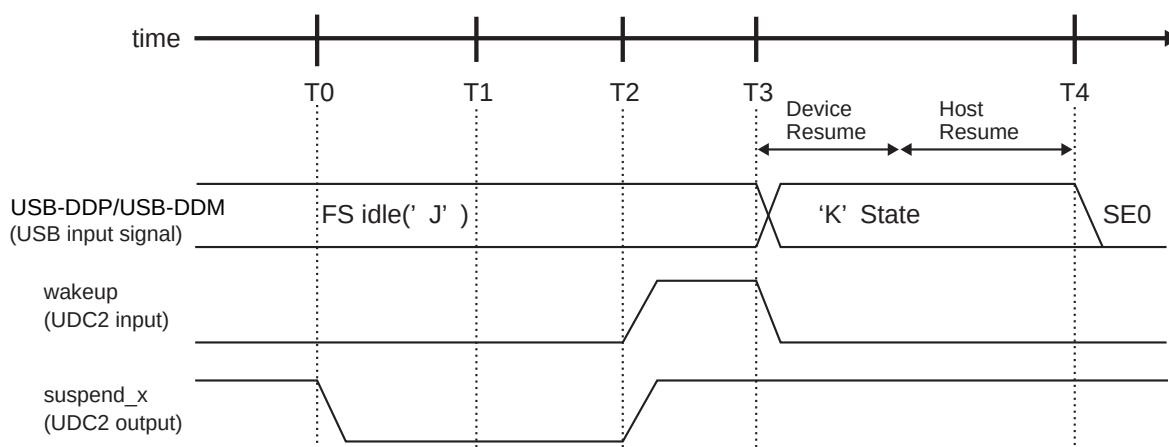
Figure 18-30 Remote wakeup operation timing
