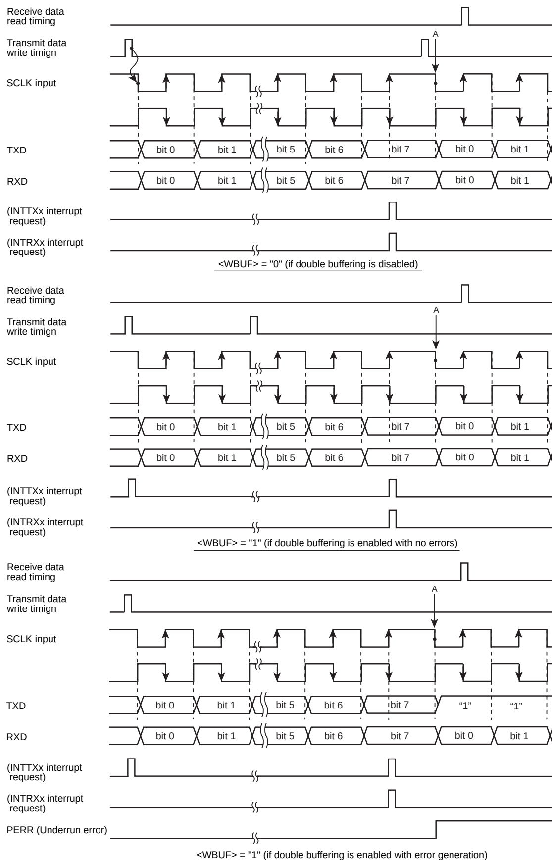
Figure 13-17 Transmit / Receive Operation in the I/O Interface Mode (SCLK Input Mode)
