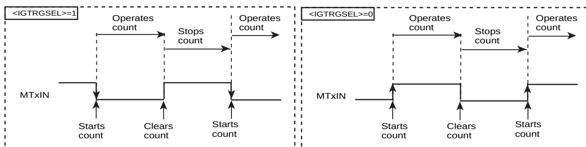
Figure 22-16 Logic of trigger input
