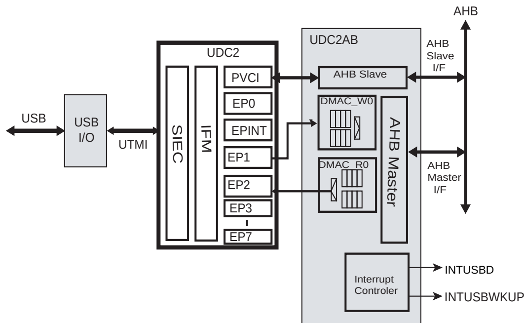
Figure 18-5 Block diagram of UDC2
