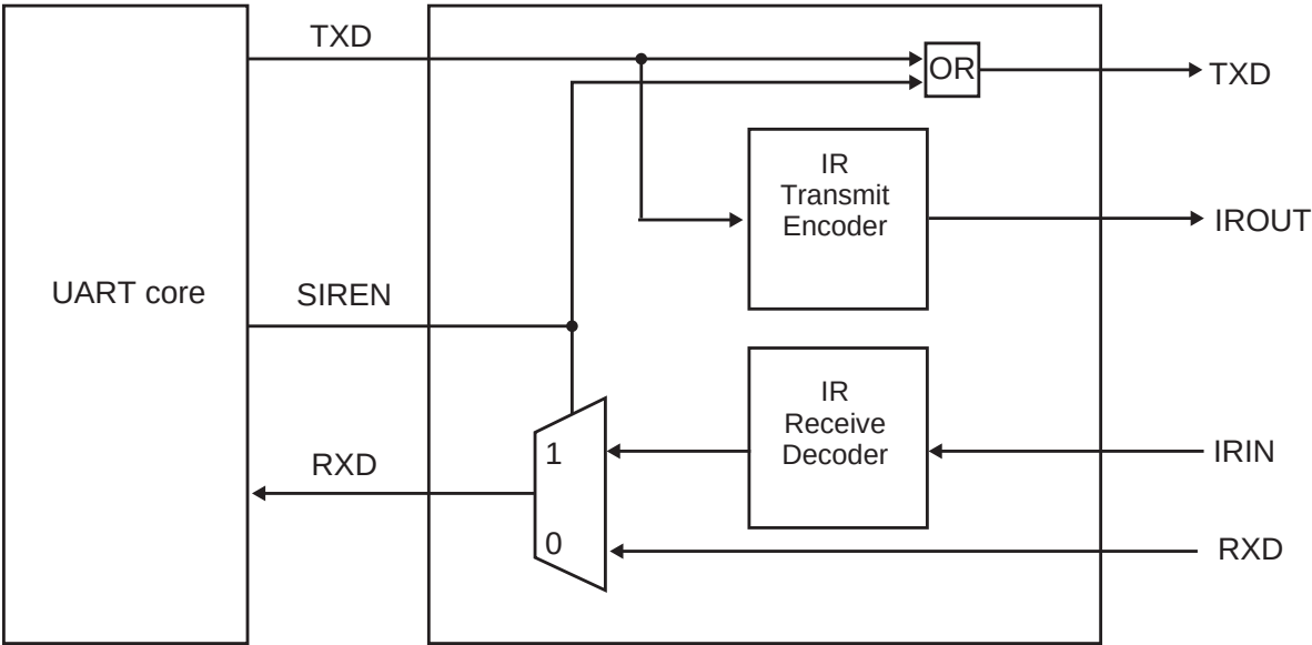
Figure 14-3 IrDA Circuit Block Diagram
