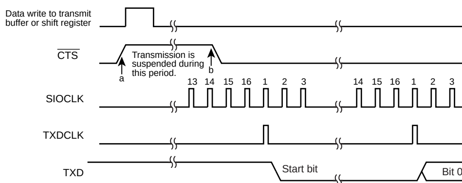
Figure 13-9 \overline{\text{CTS}} Signal timing
