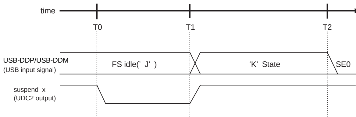
Figure 18-29 Resume operation timing by the host
