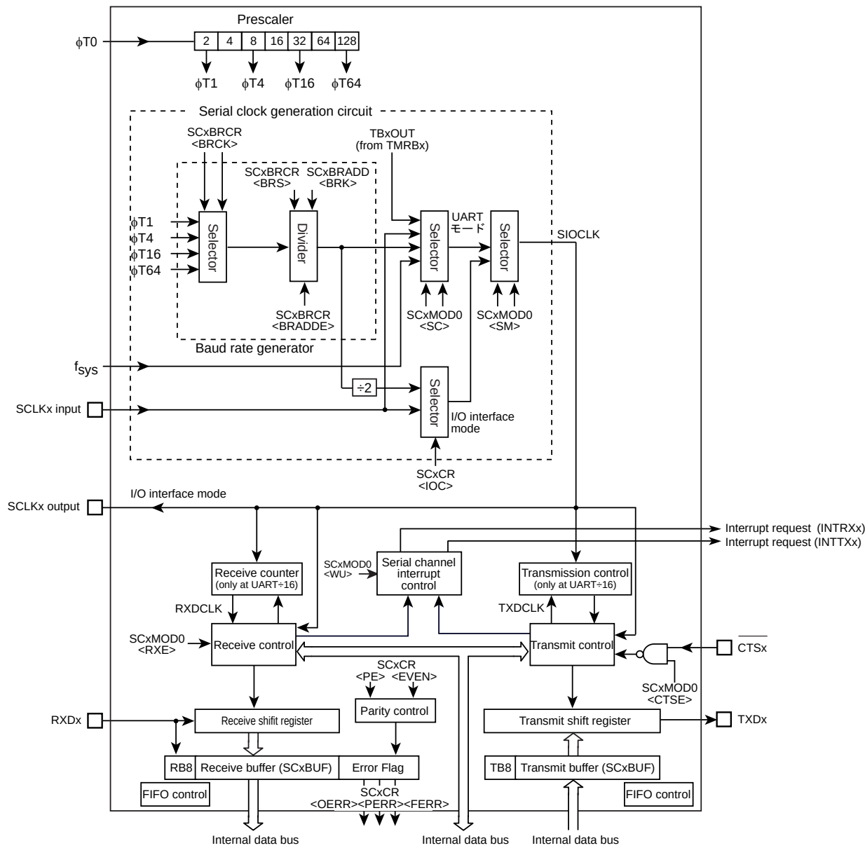
Figure 13-1 SIO / UART Block Diagram
