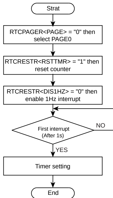
Figure 24-3 Flowchart of the clock data writing
