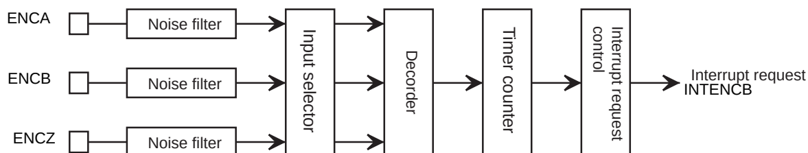
Figure 23-1 Block diagram of encoder input circuit
