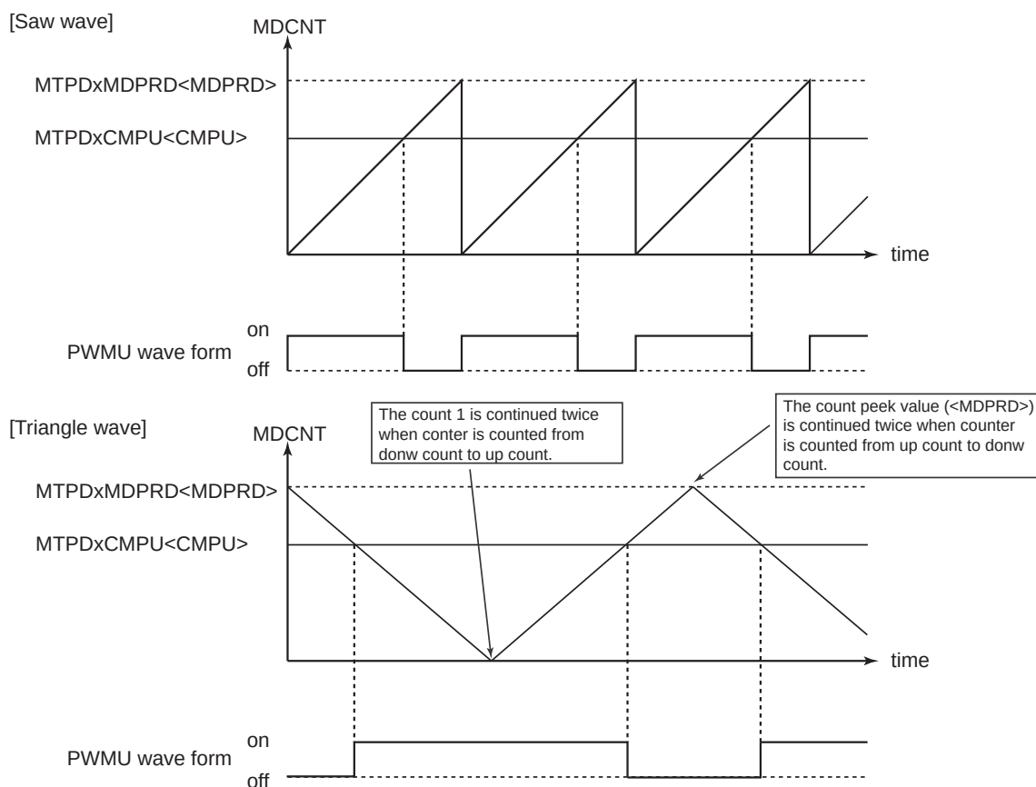
Figure 22-23 PWM waveform
