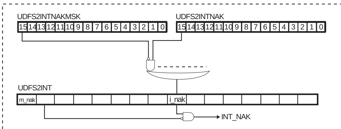
Figure 18-12 Interrupt and Status Register
