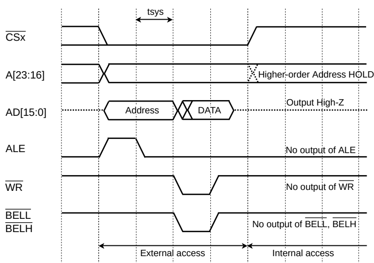
Figure 11-2 Write Operation Timing
