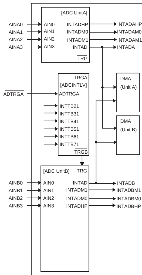
Figure 20-2 AD Converter Block Diagram
