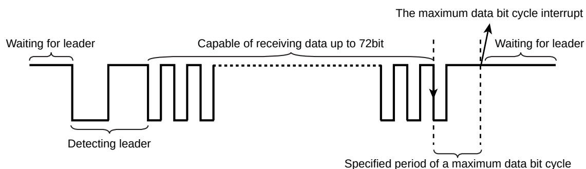
Figure 19-2 Data reception completed by detecting the max data bit cycle
