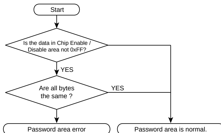
Figure 29-8 Password Area Verification Flowchart (2)
