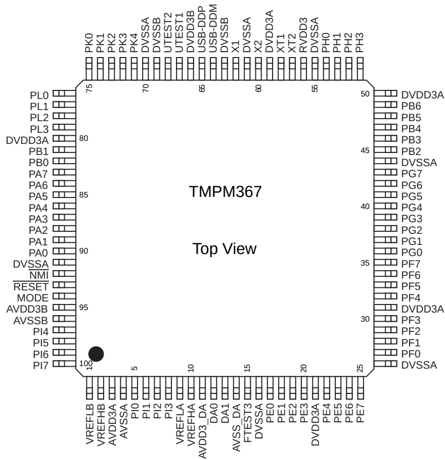
Figure 1-2 Pin Layout
