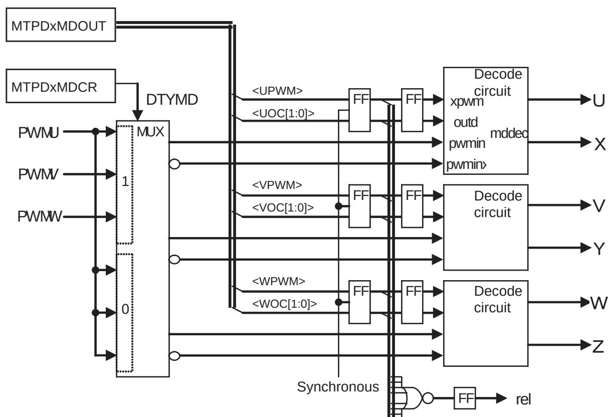
Figure 22-24 Schematic diagram of applying current control circuit
