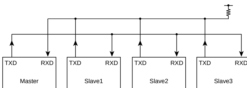
Figure 13-18 Serial Links to Use Wake-up Function
