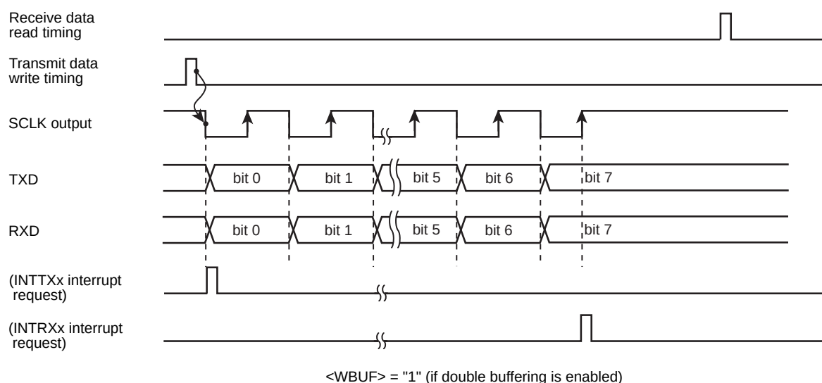
Figure 13-16 Transmit / Receive Operation in the I/O Interface Mode (SCLK Output Mode)
