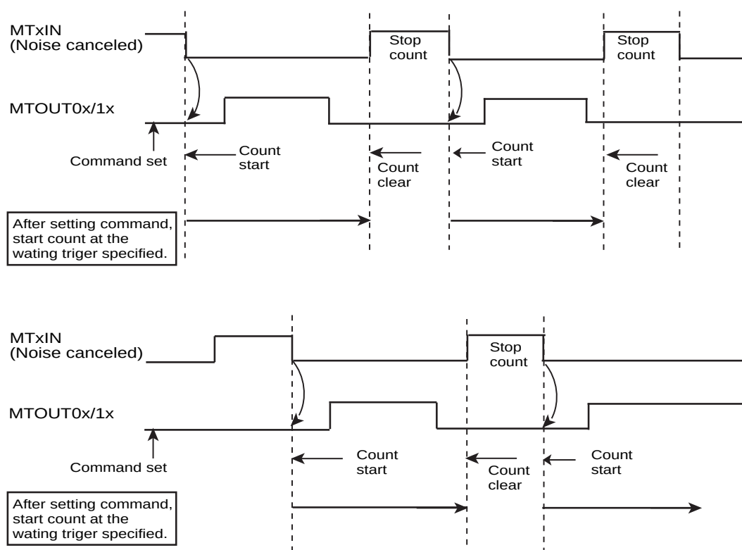
Figure 22-12 Trigger Start
