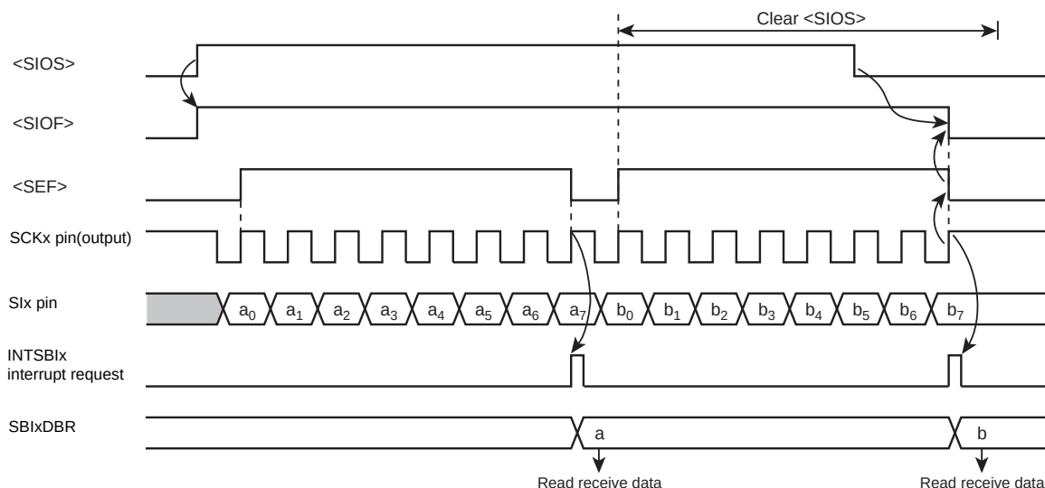
Figure 15-19 Receive Mode (Example: Internal Clock)
