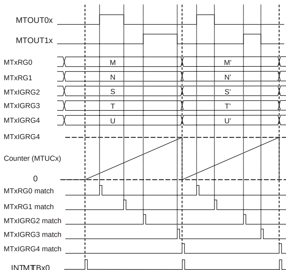
Figure 22-8 IGBT mode basic timing
