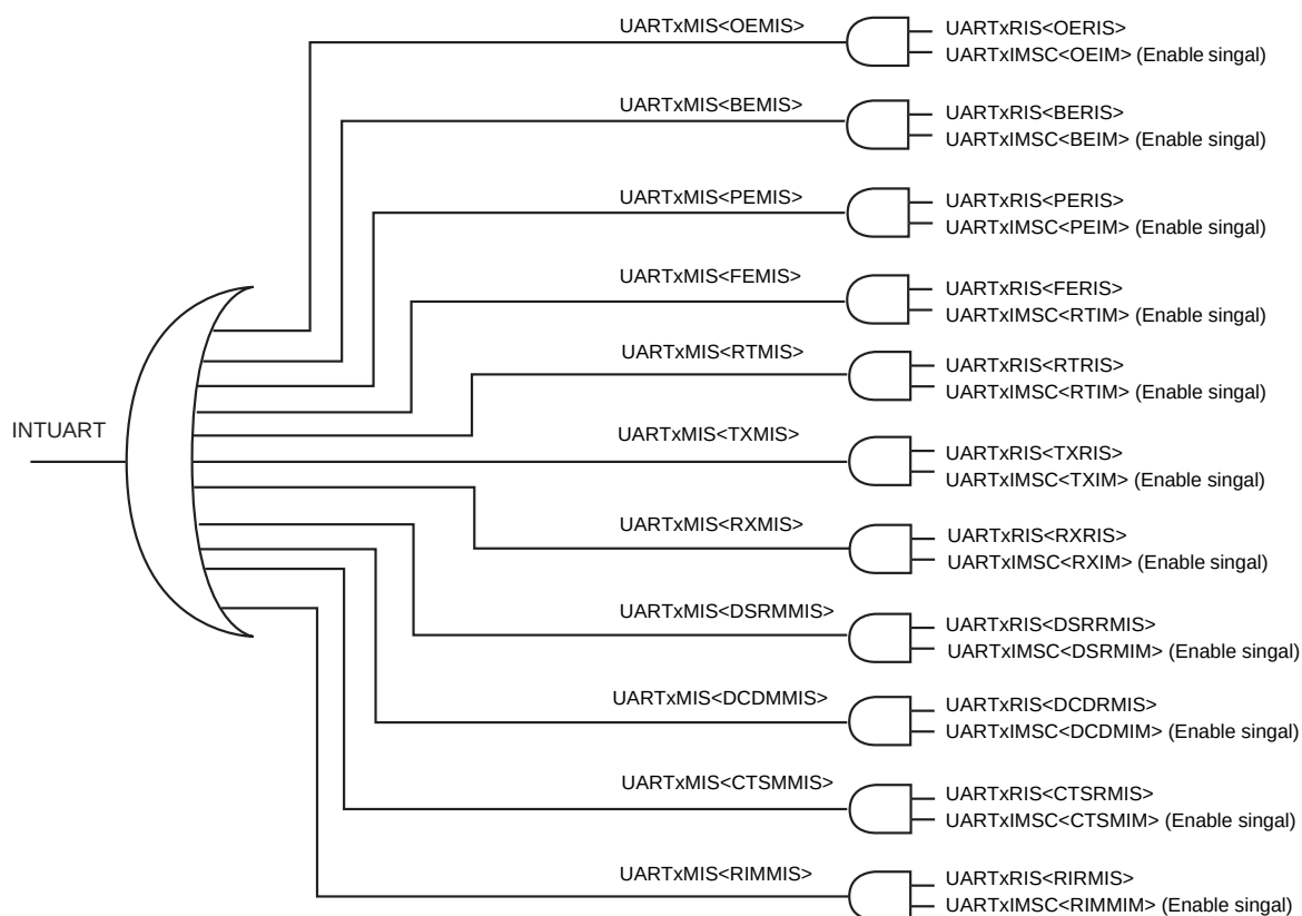
Figure 14-2 UART interrupt block
