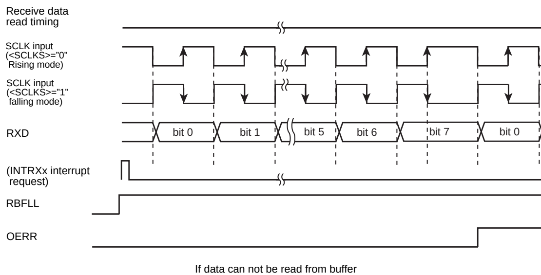
Figure 13-15 Receive Operation in the I/O Interface Mode (SCLK Input Mode)
