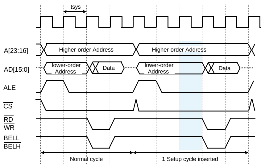
Figure 11-9 Timing of Read or Write Setup Time Insertion
