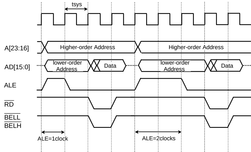
Figure 11-6 Read Operation Timing (When the ALE is 1 Clock or 2 Clocks)
