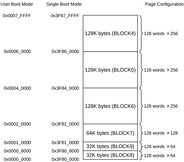
Figure 29-10 Block Configuration of Flash Memory (TMPM367FDFG)
