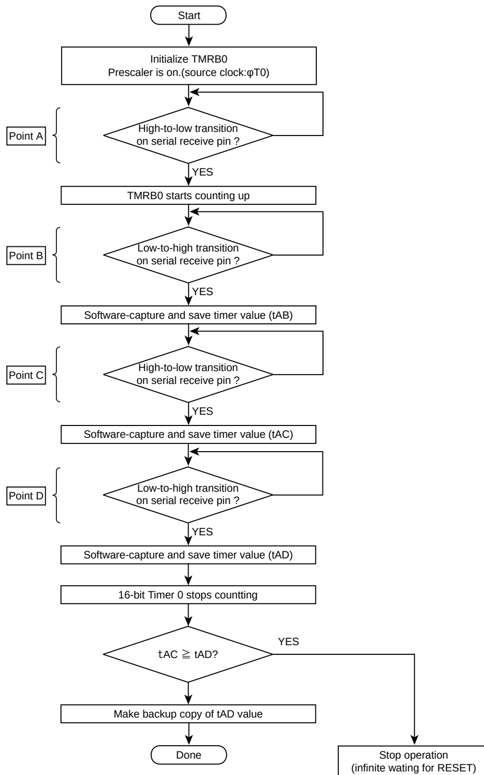
Figure 29-5 Serial Operation Mode Byte Reception Flowchart
