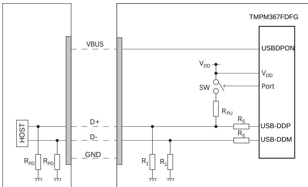
Figure 18-6 Connection example of the USB bus and TMPM367FDFG.
