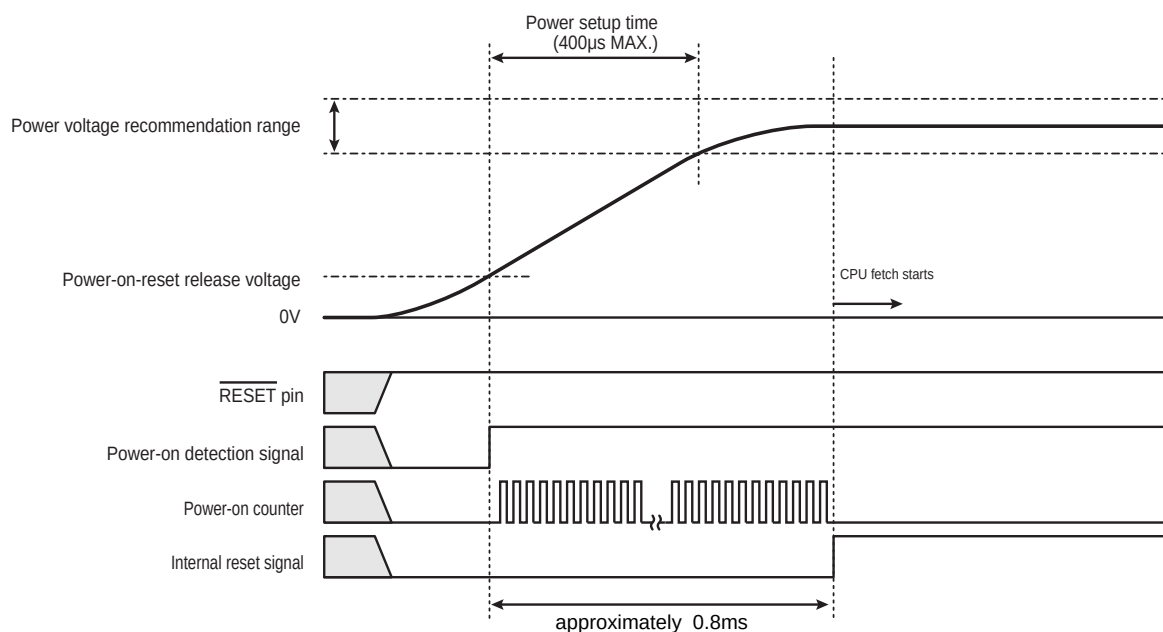
Figure 7-1 Reset Operation by Power-on Circuit
