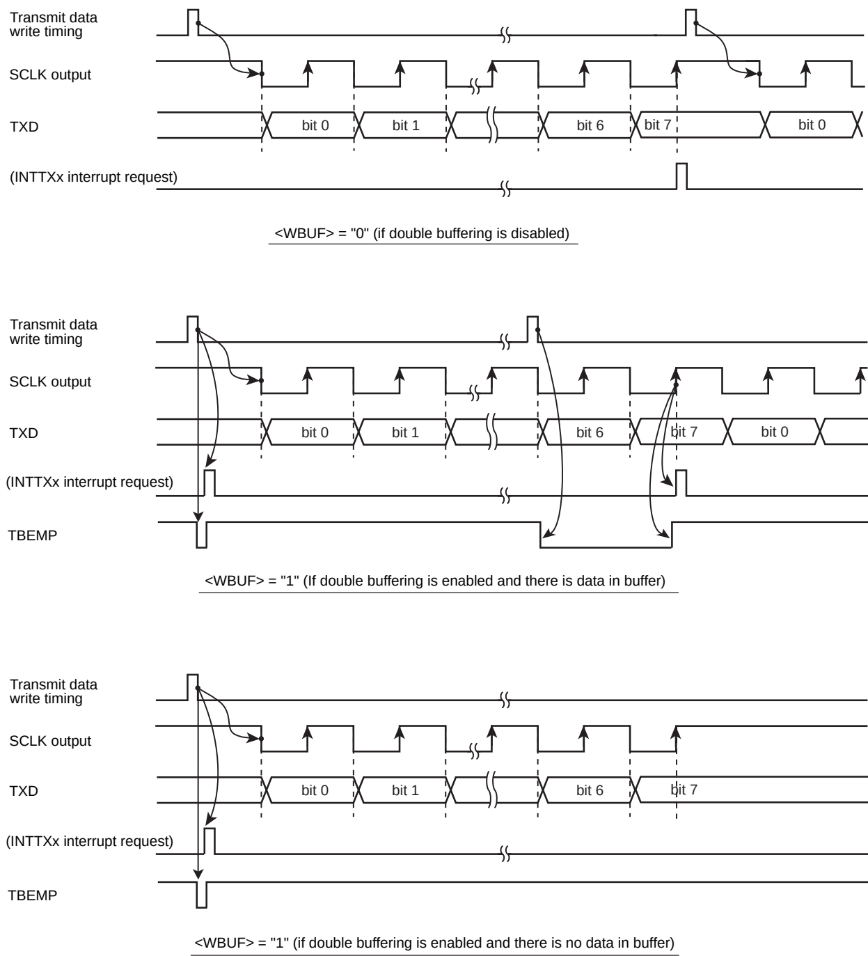
Figure 13-12 Transmit Operation in the I/O Interface Mode (SCLK Output Mode)
