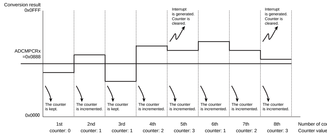
Figure 20-6 AD Monitor Function (fixed channel repeat and cumulative method)
