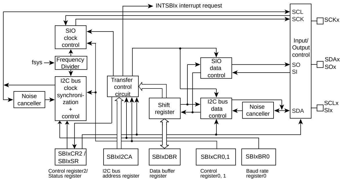
Figure 15-1 (I2C/SIO) Block Interface
