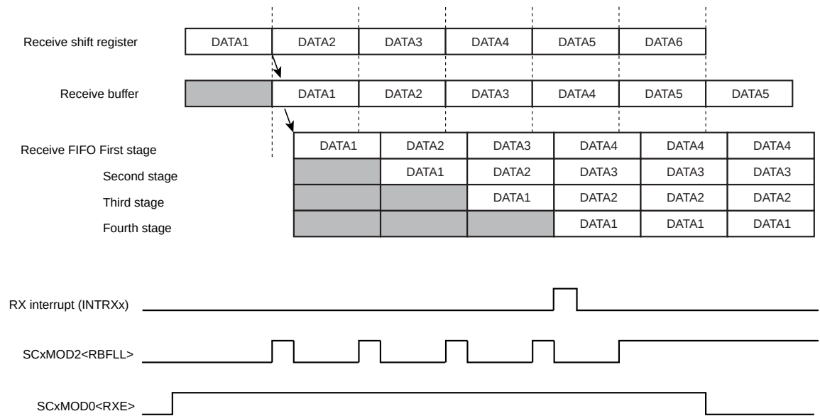
Figure 13-5 Receive FIFO Operation
