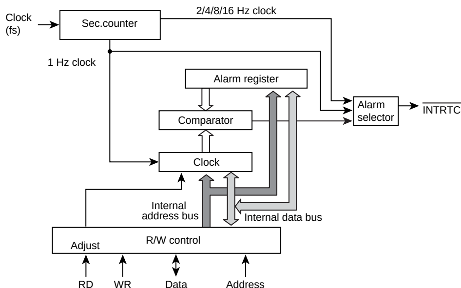
Figure 24-1 Block Diagram
