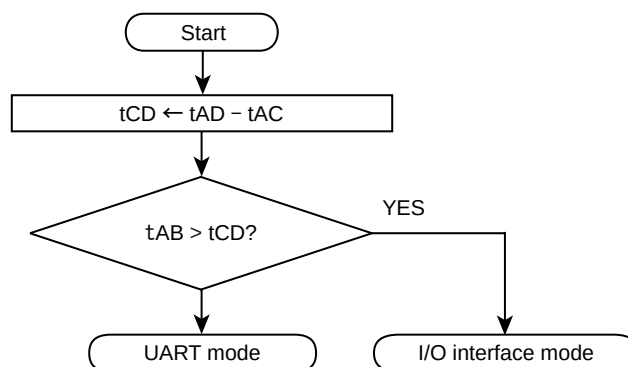
Figure 29-6 Serial Operation Mode Determination Flowchart
