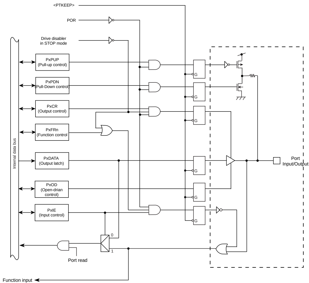
Figure 10-8 Port Type FT8
