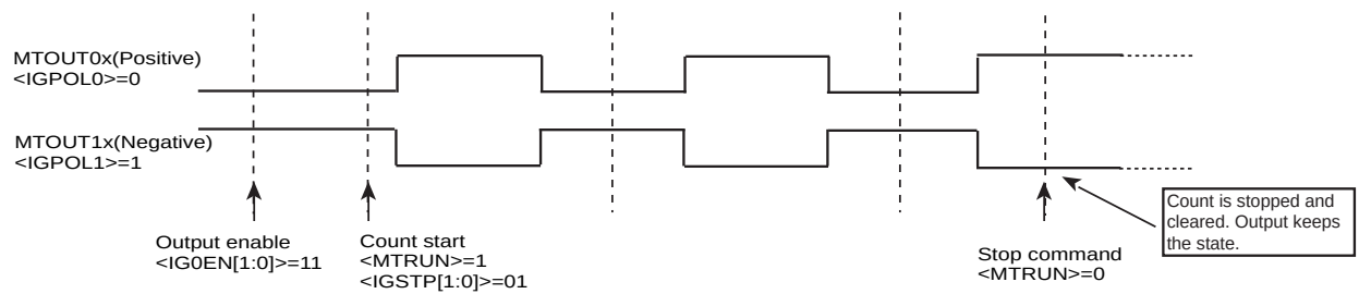
Figure 22-14 Counter stops with maintaining the output status
