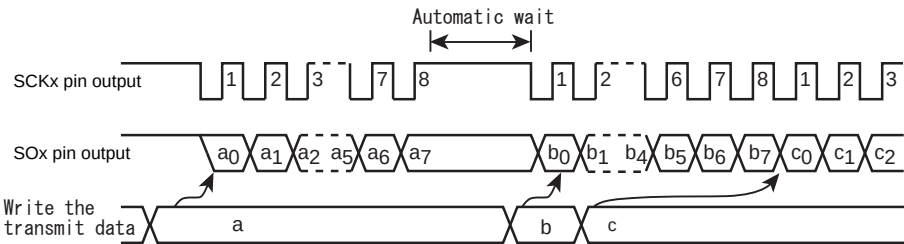
Figure 15-15 Automatic Wait
