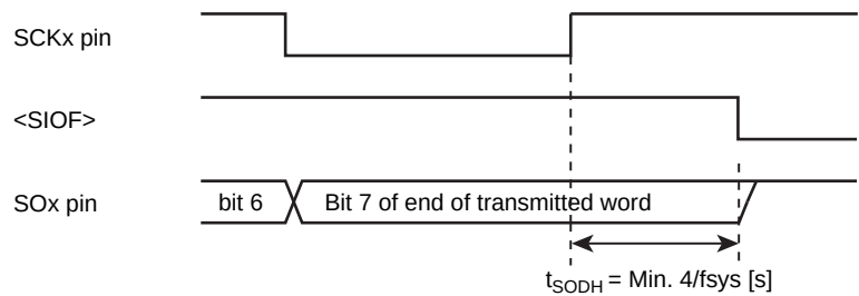
Figure 15-21 Data retention time of the last bit at the end of transmission
