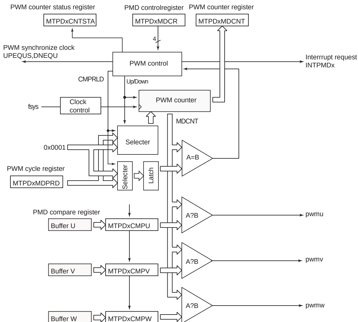
Figure 22-22 Schematic diagram of pulse width modulation circuit
