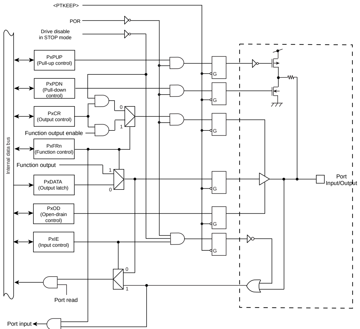
Figure 10-10 Port Type FT10
