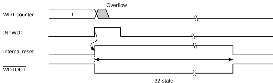
Figure 28-3 Internal reset generation
