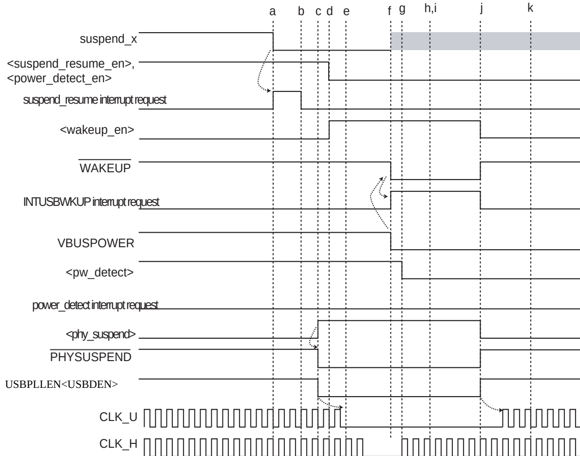
Figure 18-19 Operation of suspend/disconnect signals (to stop CLK_H)
