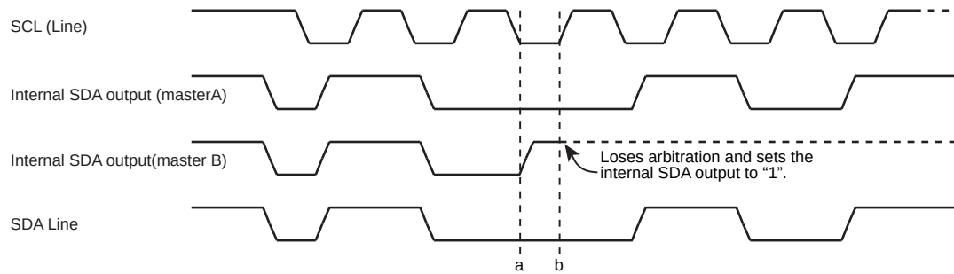
Figure 15-7 Lost Arbitration
