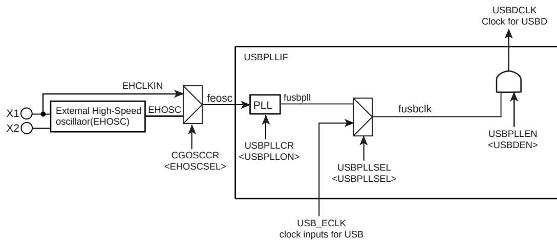
Figure 17-1 USB system diagram
