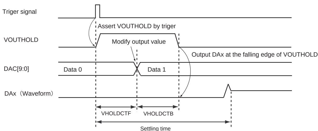
Figure 21-4 VOUTHOLD and settling time
