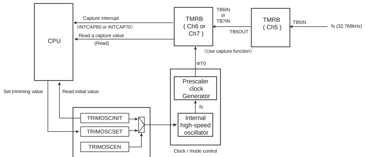
Figure 5-2 The way of input fs into TB5IN
