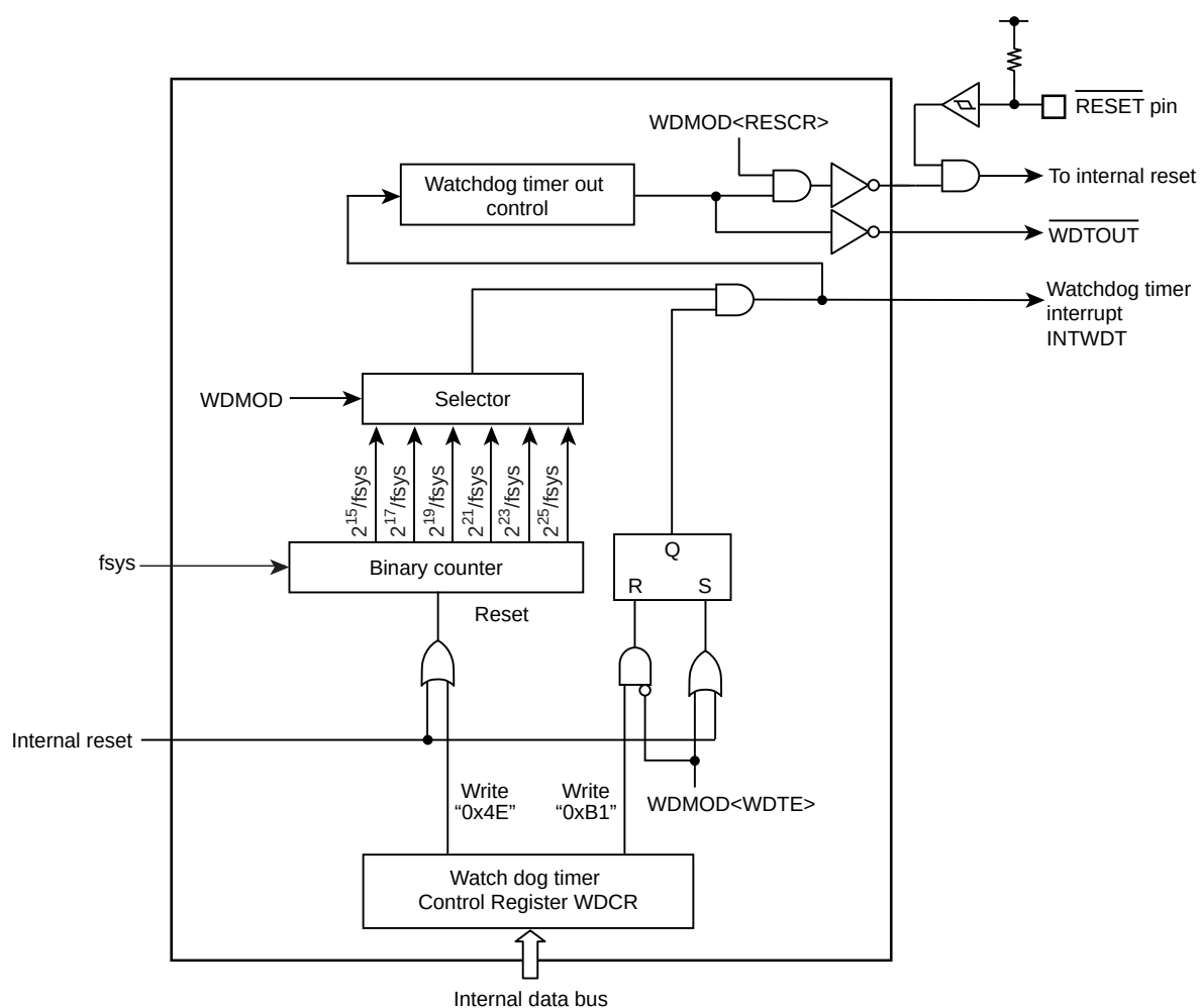
Figure 28-1 Block Diagram of the Watchdog Timer
