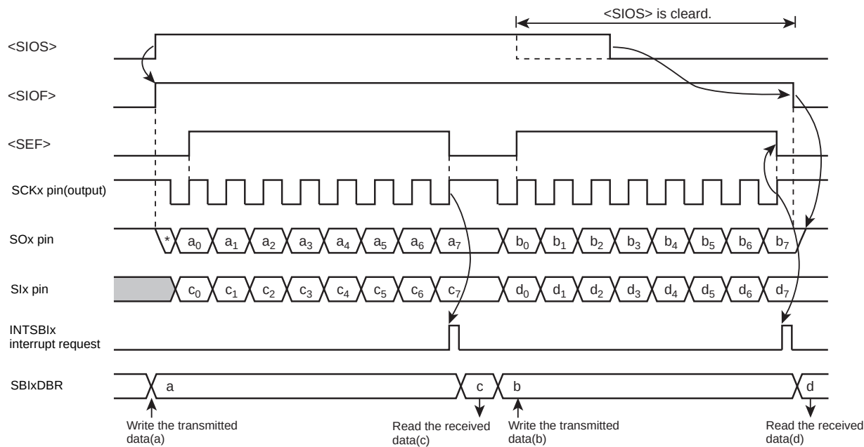
Figure 15-20 Transmit/Receive Mode (Example: Internal Clock)
