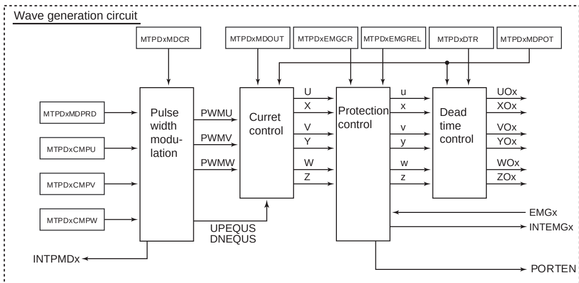
Figure 22-21 Schematic diagram of PMD circuit
