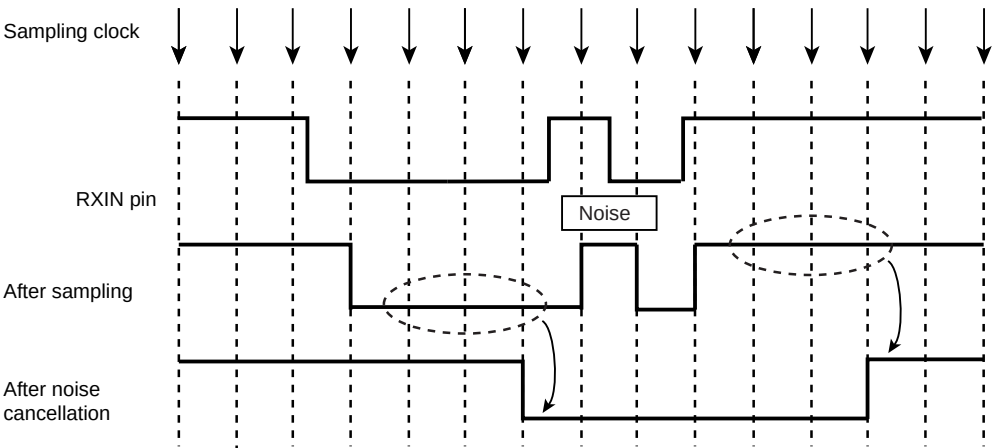
Figure 19-3 Noise Cancel (In the case of RMCRCR4="0011" (3 Cycles))
