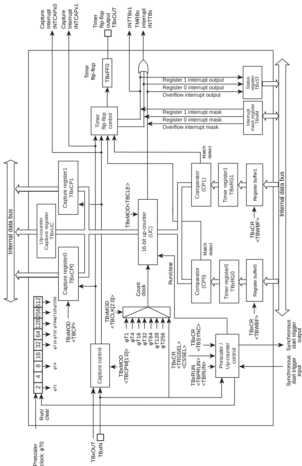
Figure 12-1 TMRBx Block Diagram
