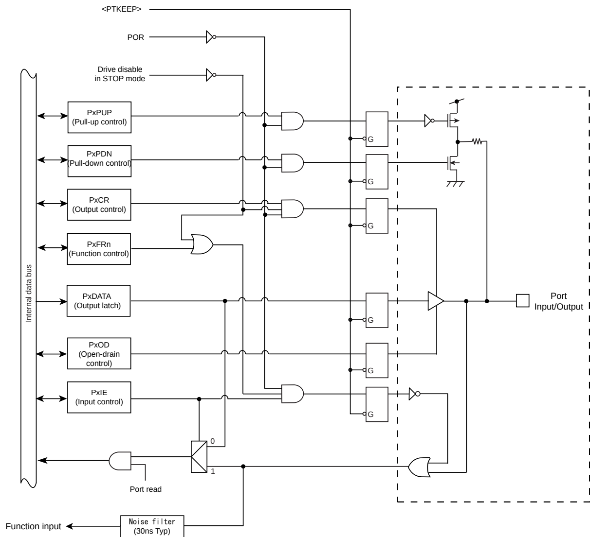
Figure 10-4 Port Type FT4
