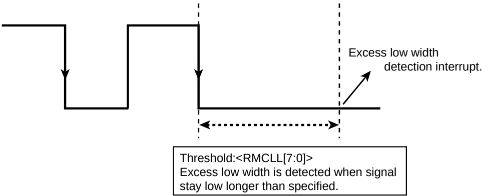
Figure 19-7 Completion by detecting low width
