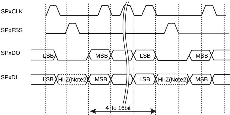
Figure 16-5 SPI frame format (continuous transfer, \langle \text{SPO} \rangle = "0" & \langle \text{SPH} \rangle = "0" )
