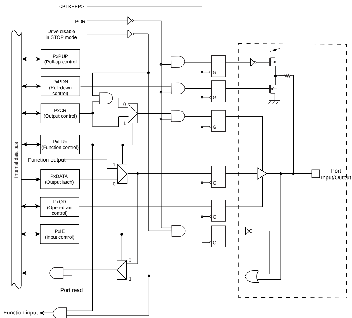
Figure 10-9 Port Type FT9
