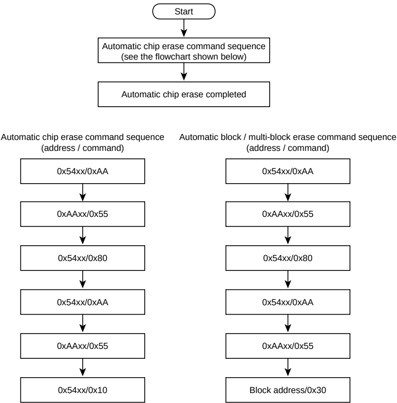
Figure 29-12 Automatic Erase
