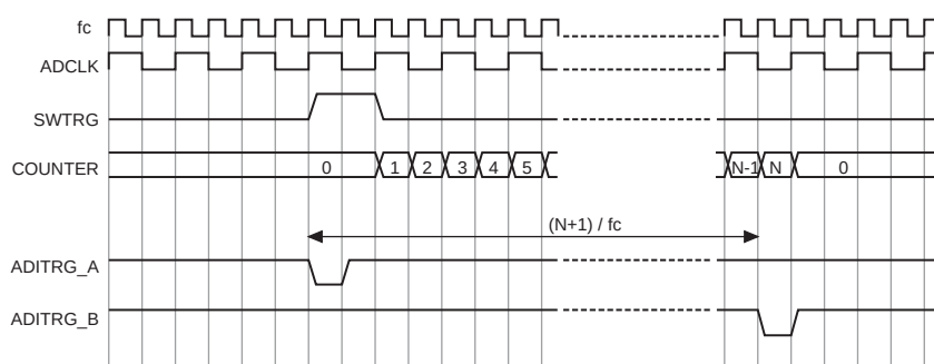
Figure 20-7 Interleave operation using a software trigger (ADCLK=fc/2)
