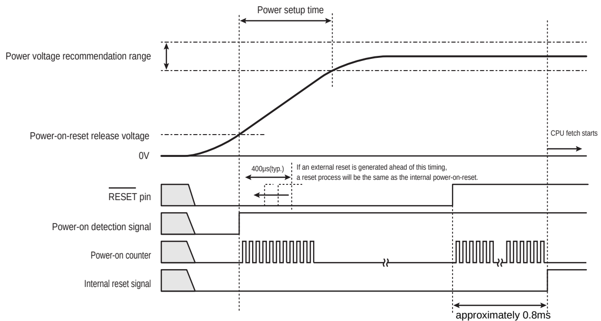
Figure 7-2 Reset Operation by \overline{\text{RESET}} pin
