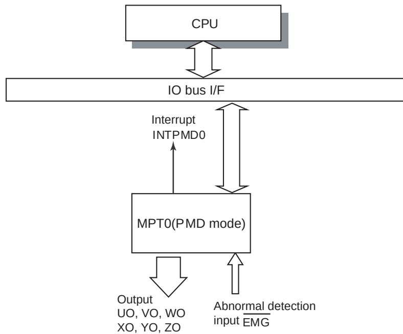
Figure 22-20 Block diagram of related with motor control
