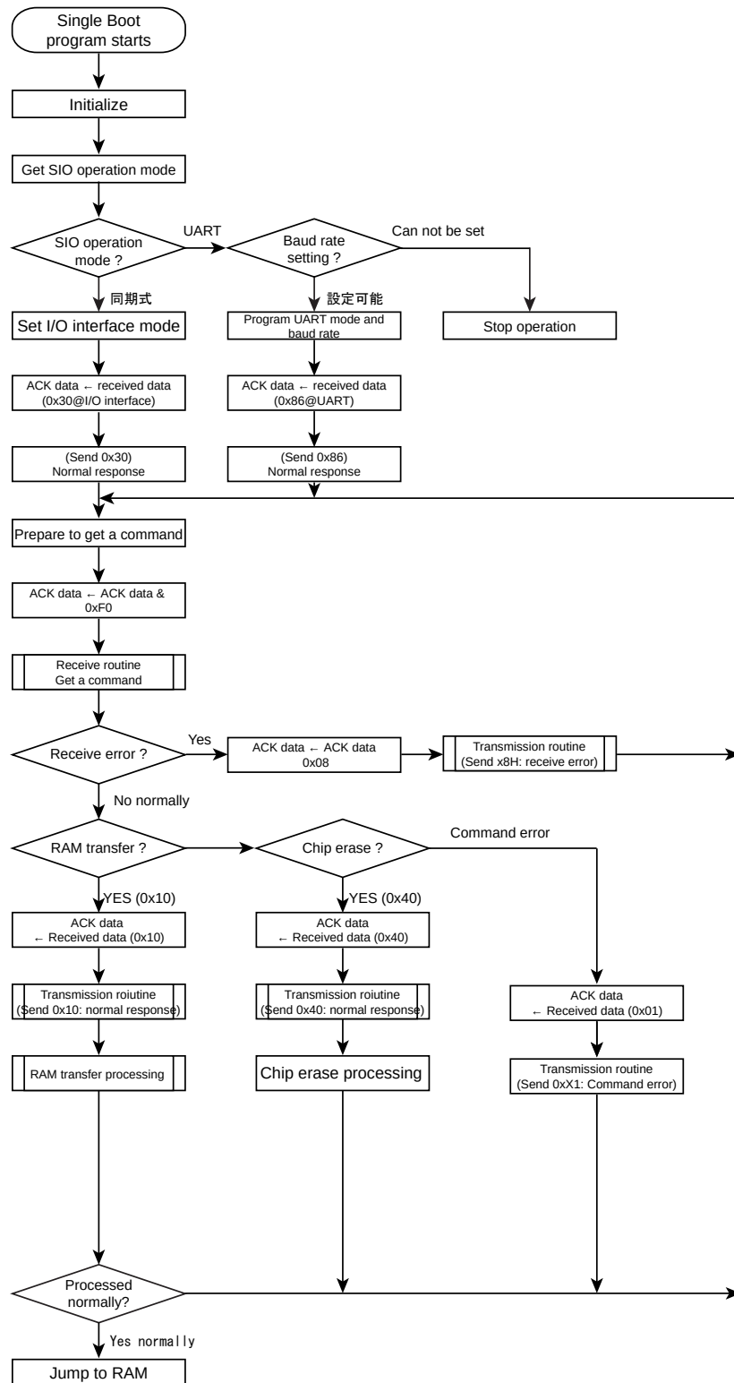
Figure 29-9 Overall Boot Program Flowchart
