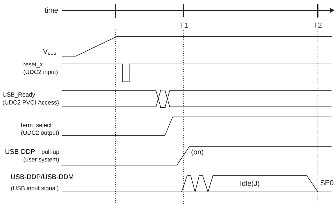
Figure 18-26 Connect operation timing
