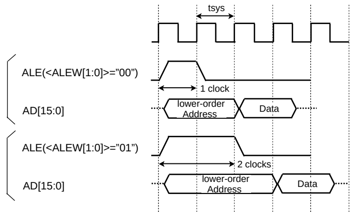
Figure 11-5 Time that it takes before ALE is asserted
