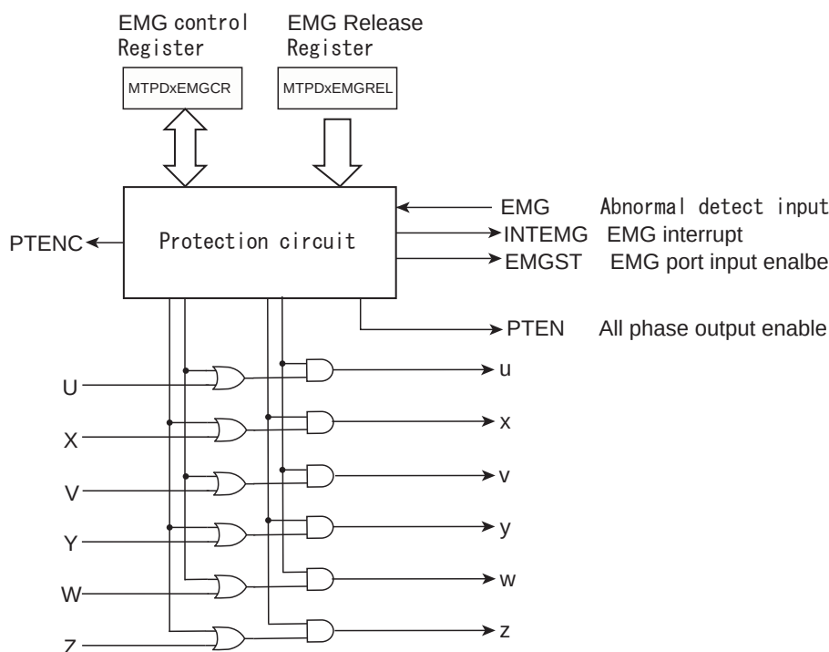
Figure 22-25 Schematic diagram of protection control circuit
