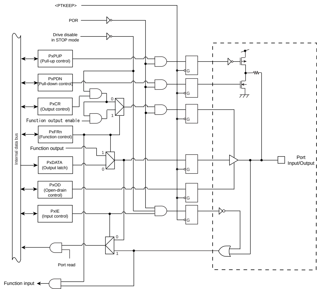
Figure 10-3 Port Type FT3
