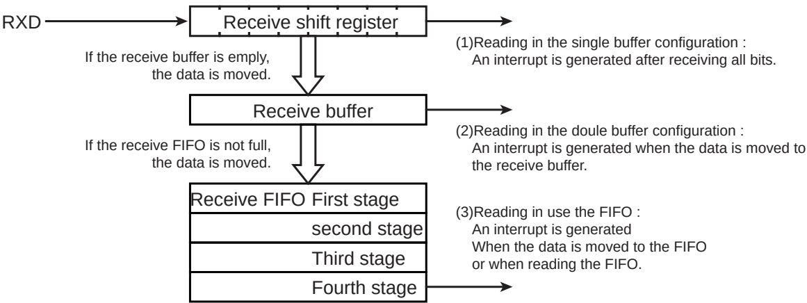
Figure 13-10 Receive Buffer / FIFO Configuration Diagram
