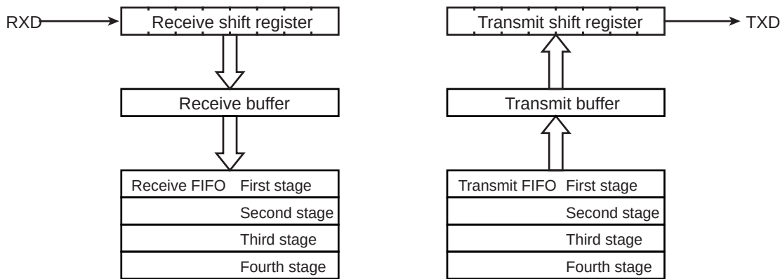
Figure 13-3 The Configuration of Buffer and FIFO
