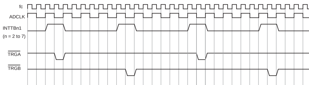
Figure 20-9 Trigger Start Operation by Timer Trigger ( ADCLK = f_c/2 )
