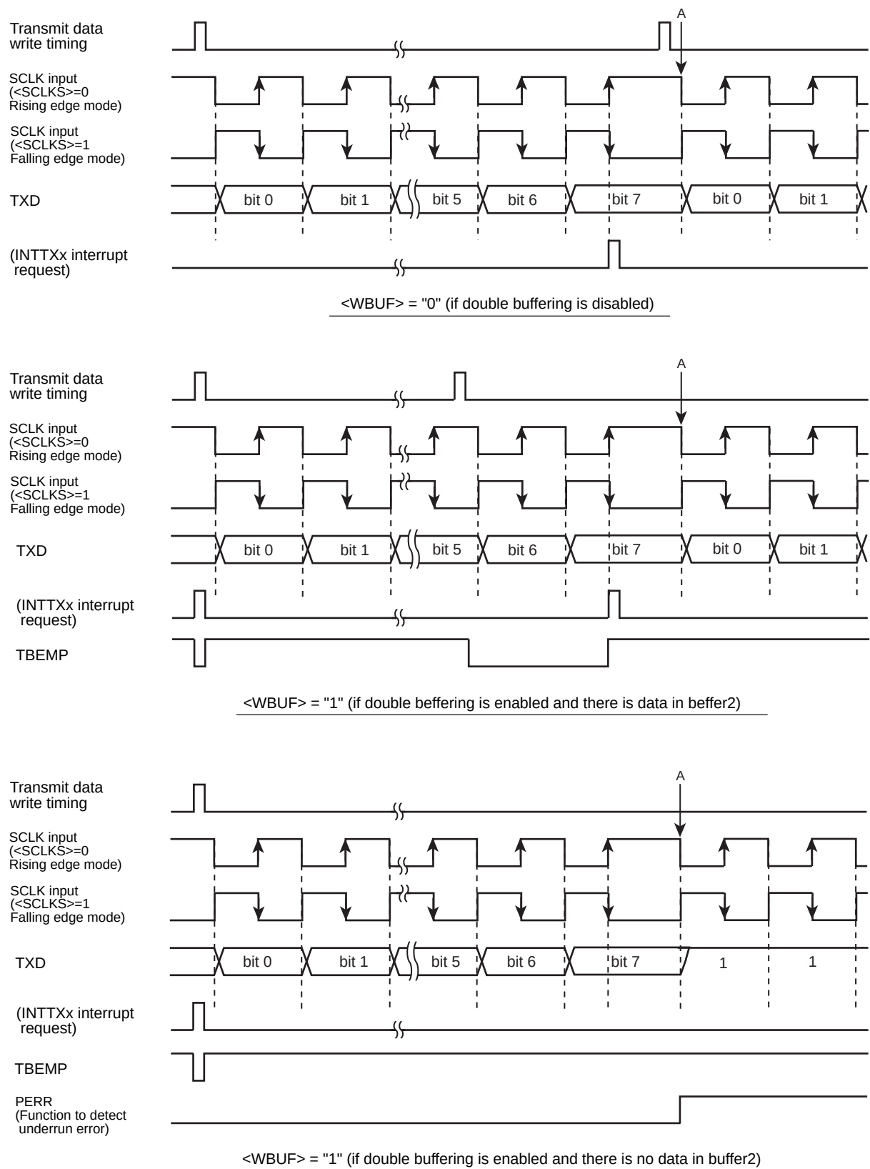
Figure 13-13 Transmit Operation in the I/O Interface Mode (SCLK Input Mode)
