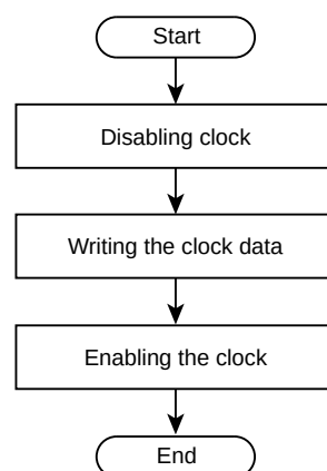
Figure 24-4 Flowchart of the disabling clock
