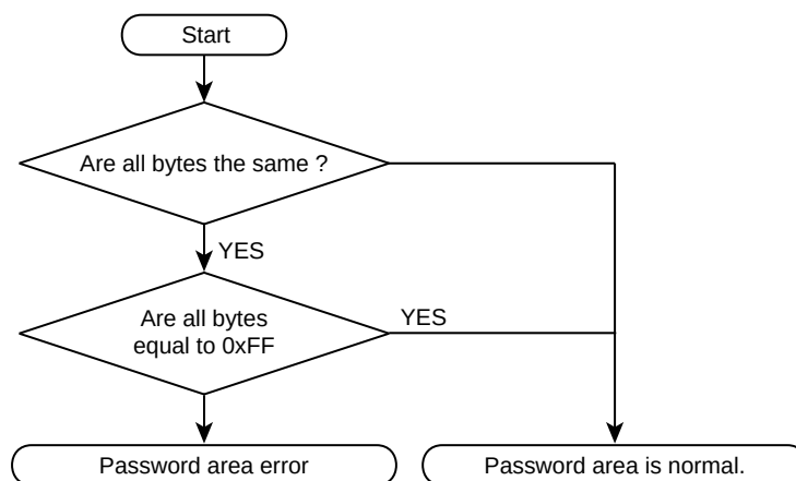
Figure 29-7 Password Area Verification Flowchart (1)
