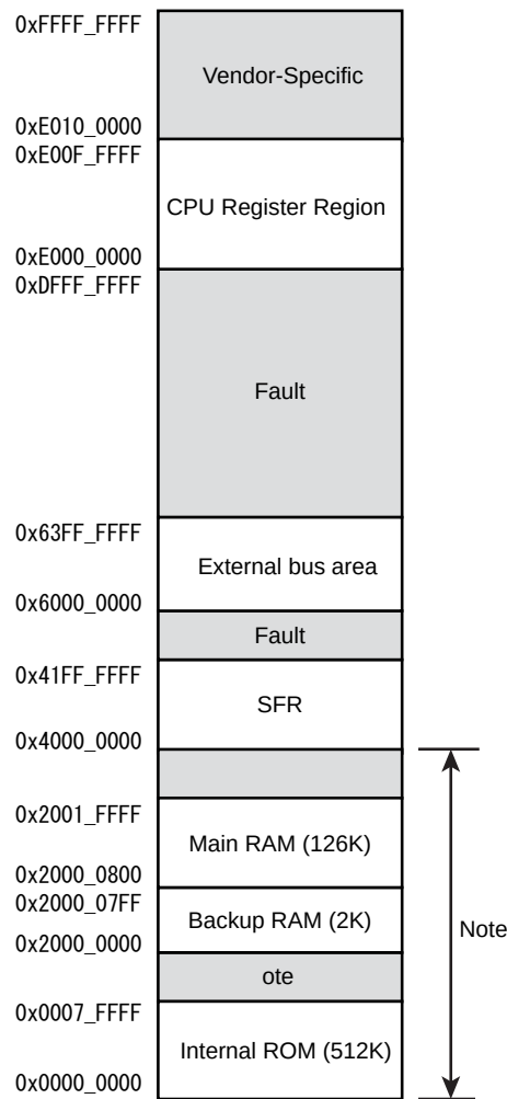
Figure 3-1 Memory Map
