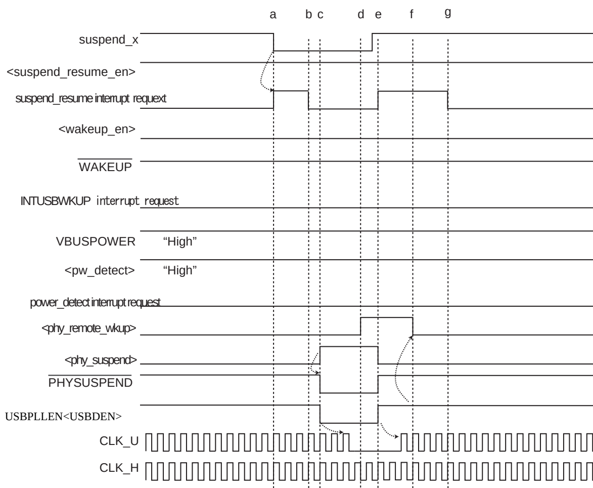
Figure 18-20 Operation of suspend/remote wakeup signals
