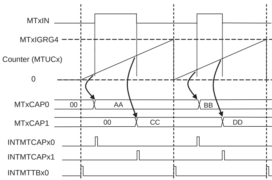
Figure 22-10 Capture operation
