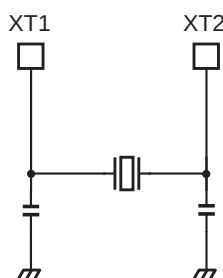
Figure 33-2 Low-frequency oscillation connection
