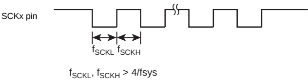
Figure 15-16 Maximum Transfer Frequency of External Clock Input
