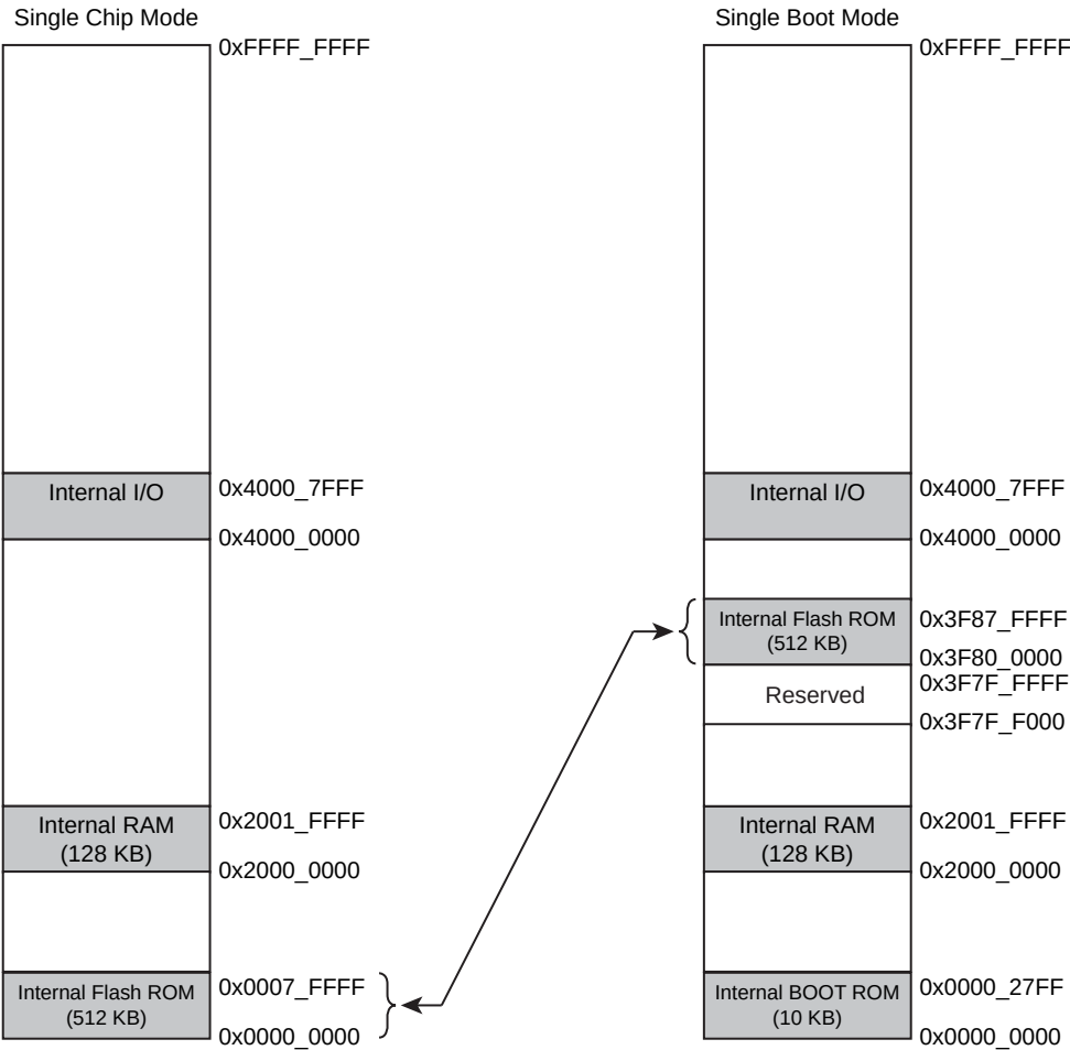
Figure 29-3 Memory Maps for TMPM367FDFG
