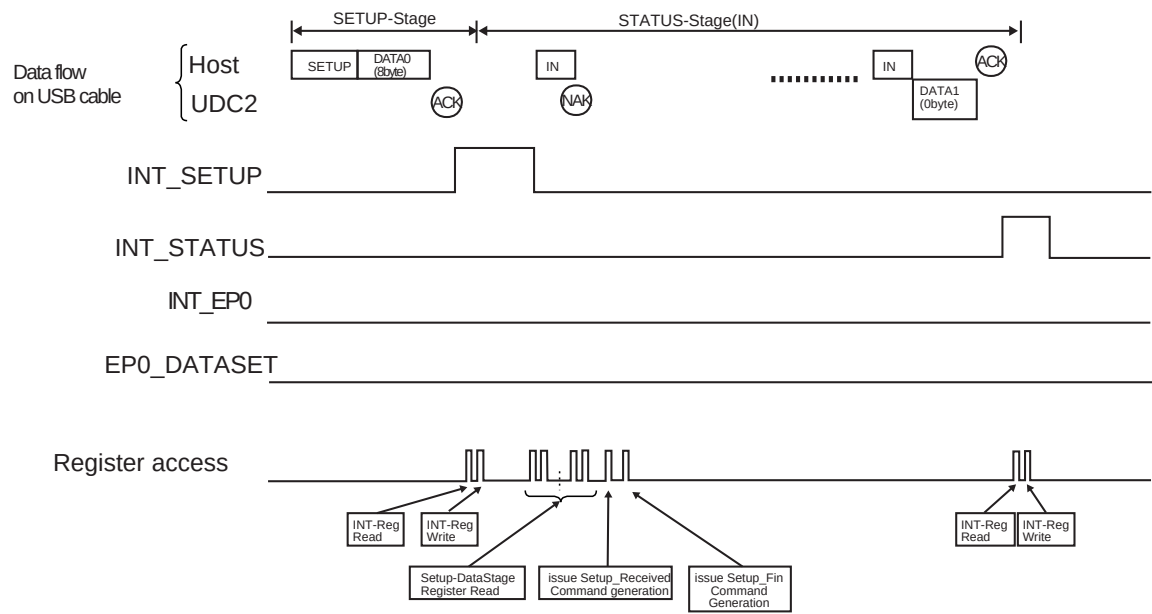
Figure 18-23 Flow of control in Control-WR transfer (without DATA-Stage)
