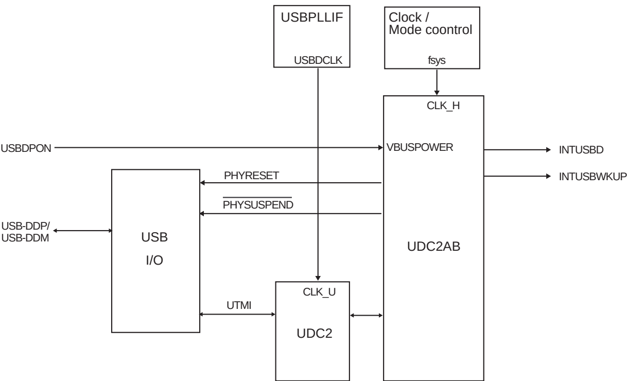
Figure 18-16 Connection Diagram of Power Management Control Signal
