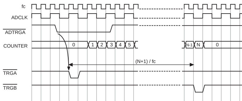
Figure 20-8 Interleave operation using an external trigger ( ADCLK=fc/2 )
