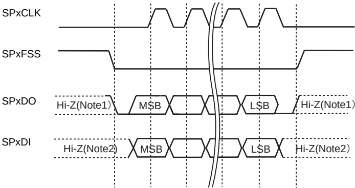
Figure 16-4 SPI frame format (single transfer, \langle \text{SPO} \rangle = "0" & \langle \text{SPH} \rangle = "0" )
