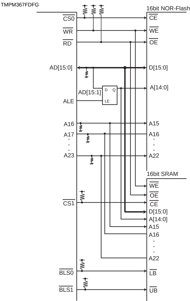
Figure 11-10 Connection Example for external 16-bit SRAM and NOR-Flash (Multiplex bus)
