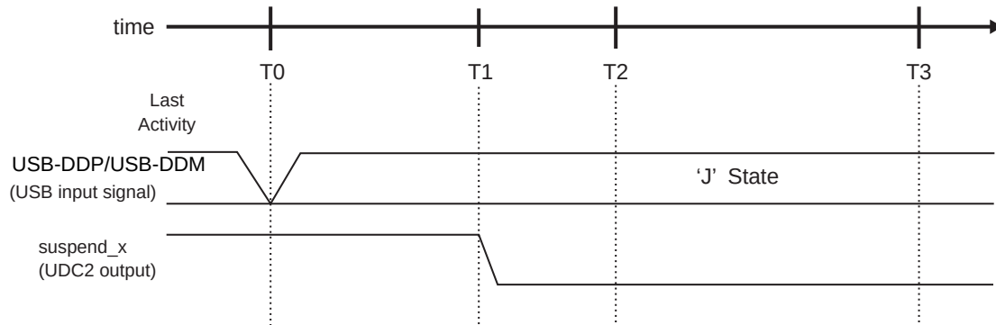
Figure 18-28 Suspend operation timing
