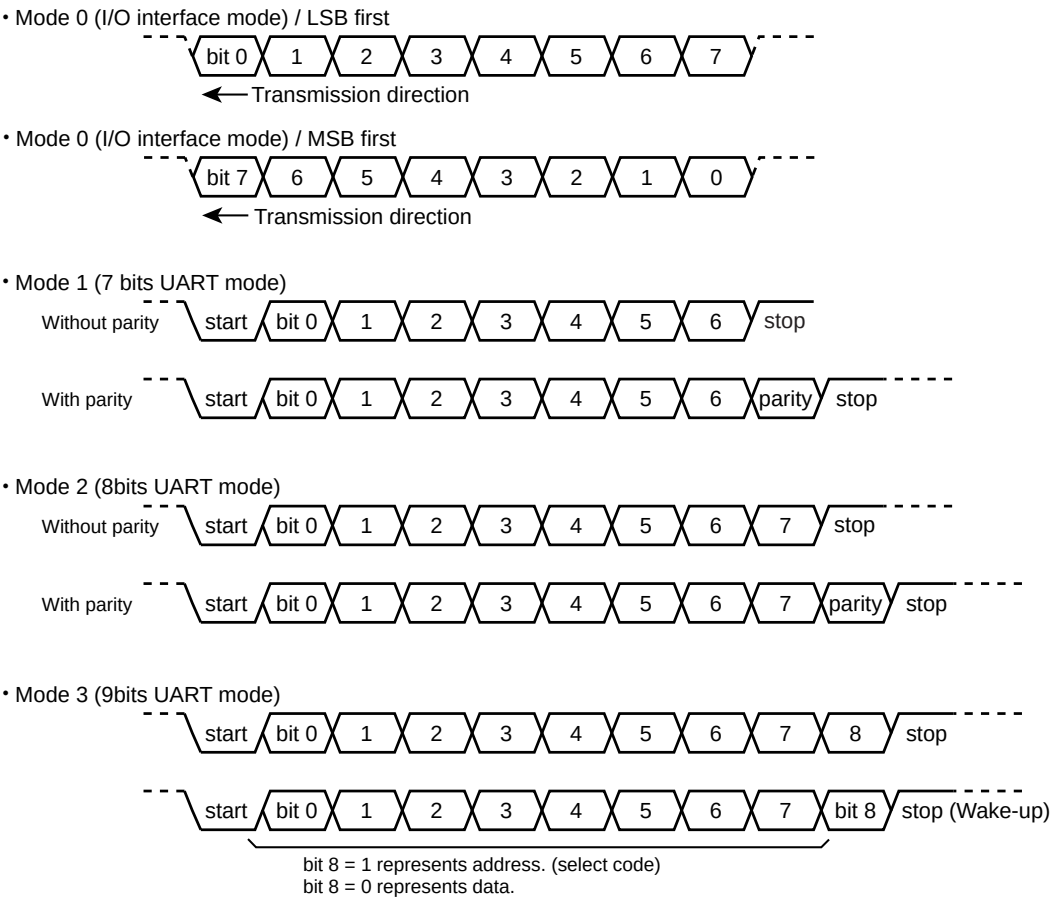
Figure 13-2 Data Format
