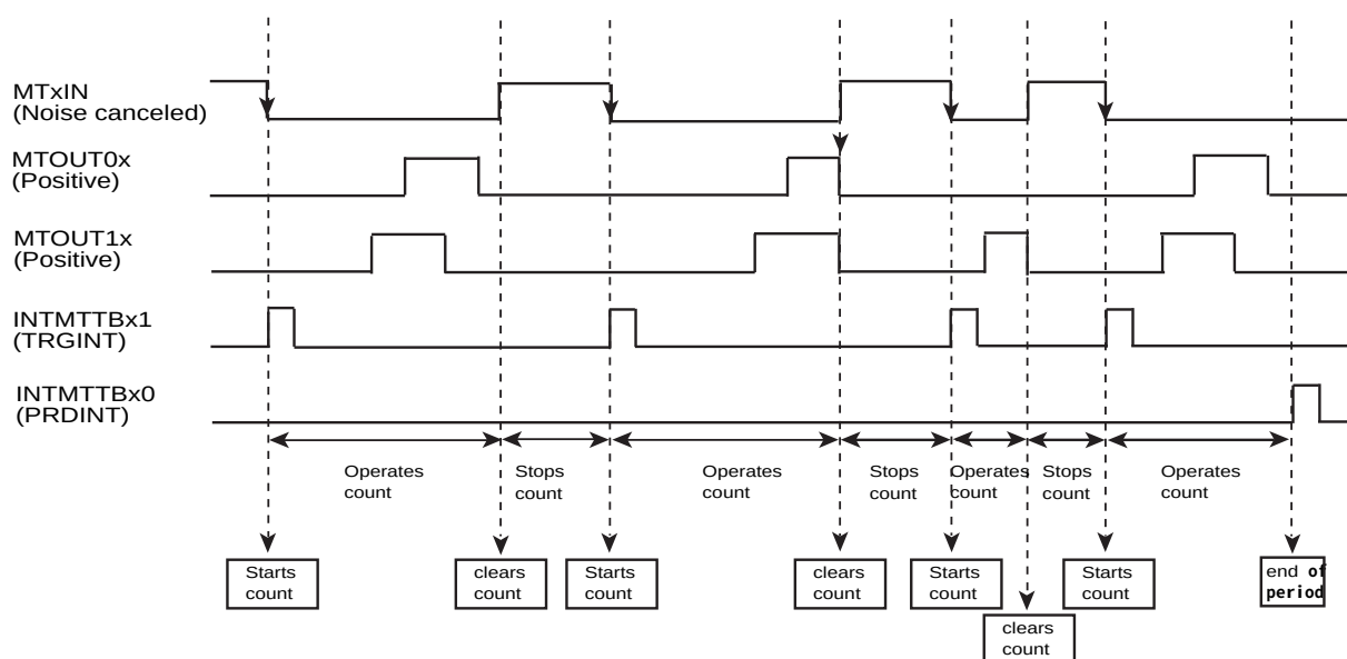
Figure 22-18 Trigger constant acceptance
