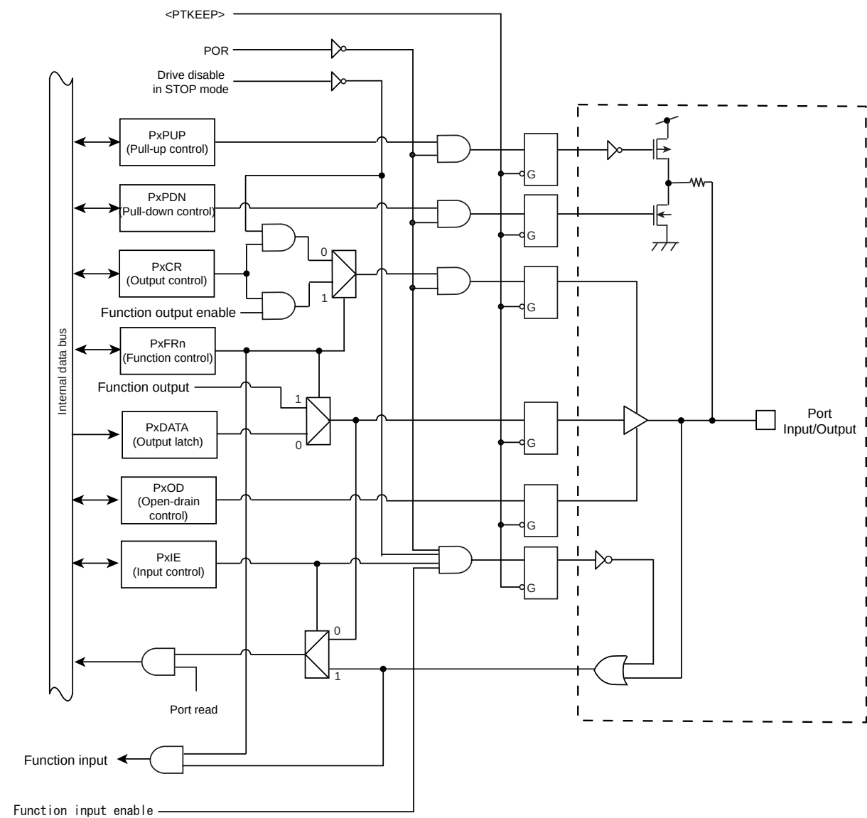
Figure 10-7 Port Type FT7
