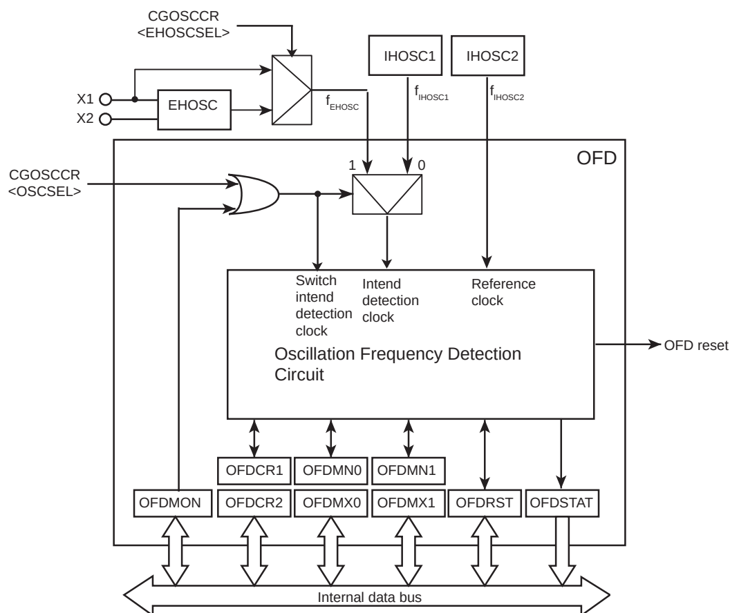
Figure 27-1 Oscillation Frequency Detector Block diagram
