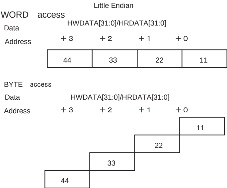
Figure 18-3 Image of Endian conversion in AHB Master function
