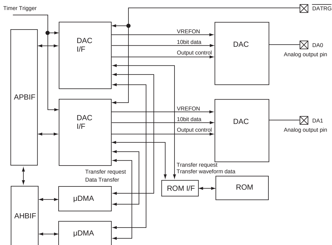
Figure 21-1 Block diagram of DAC
