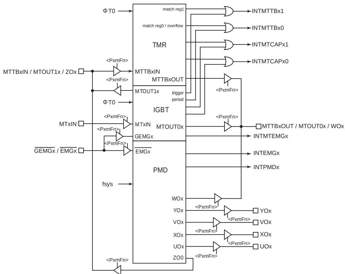
Figure 22-1 Block Diagram of MPTx
