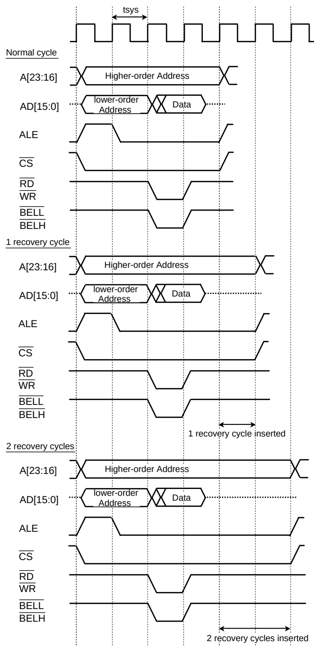
Figure 11-7 Timing of Recovery Time Insertion
