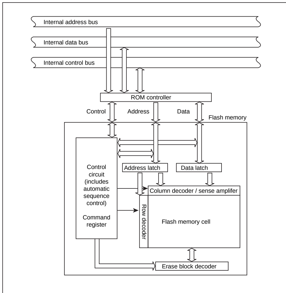
Figure 29-1 Block Diagram of the Flash Memory Section
