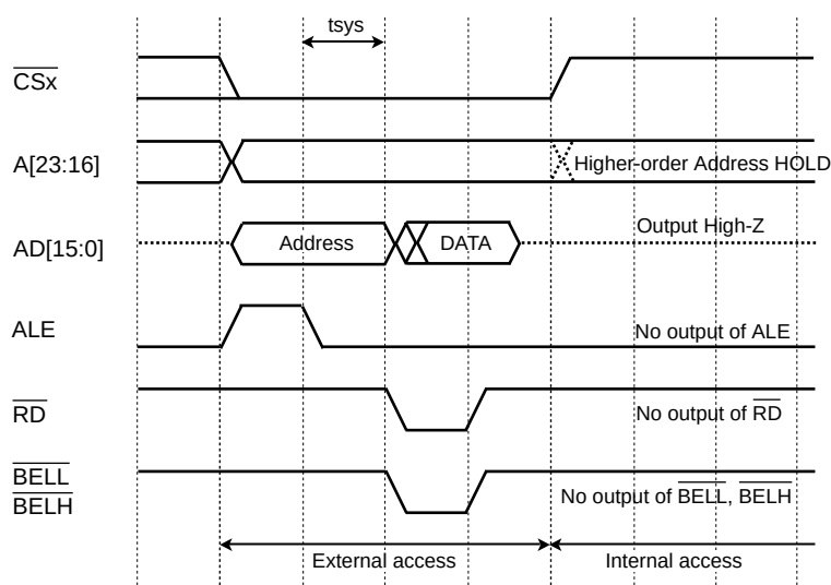
Figure 11-1 Read Operation Timing
