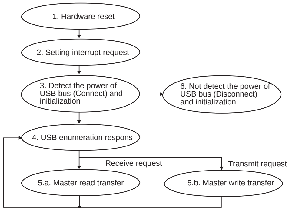
Figure 18-14 Operation Sequence
