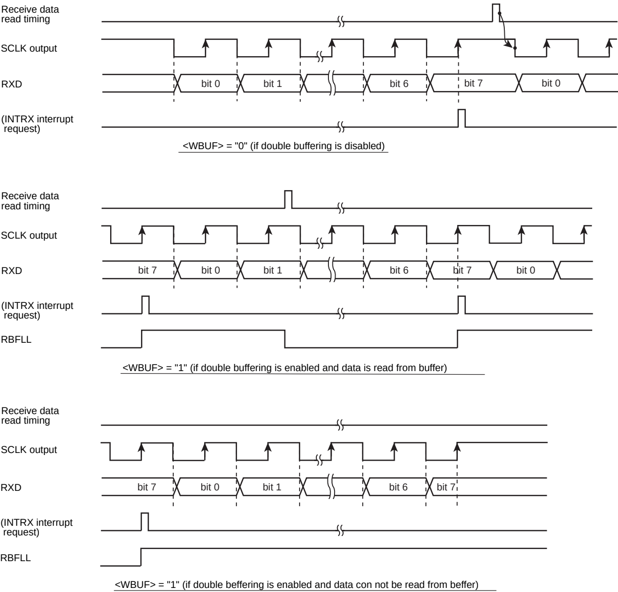
Figure 13-14 Receive Operation in the I/O Interface Mode (SCLK Output Mode)
