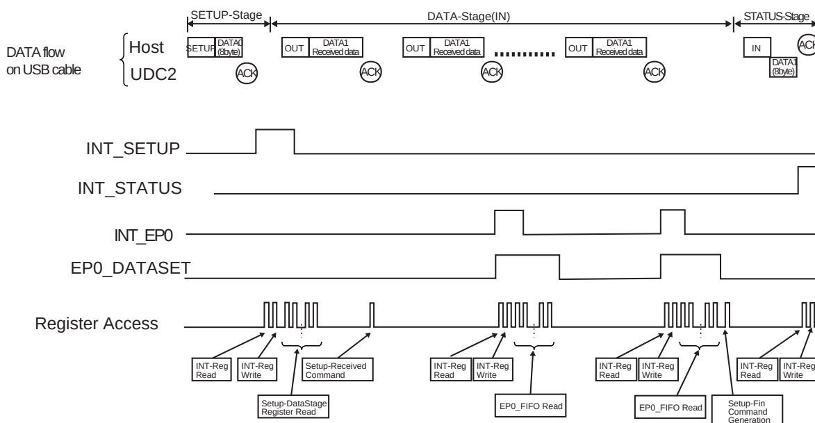
Figure 18-24 Flow of control in Control-WR transfers (with DATA-Stage)
