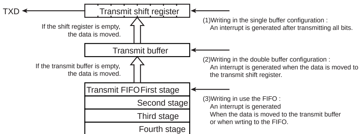
Figure 13-11 Transmit Buffer / FIFO Configuration Diagram
