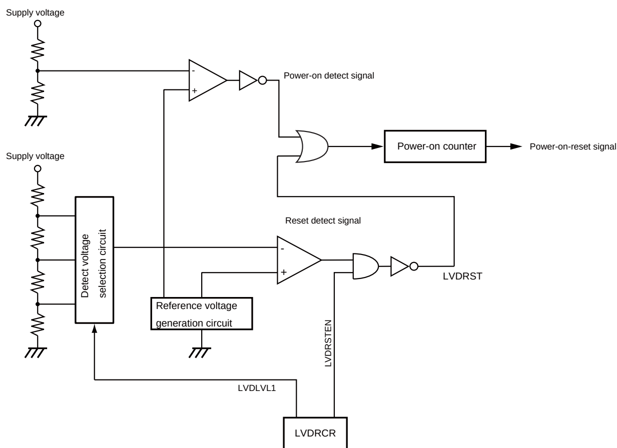
Figure 25-1 Power-on-reset circuit
