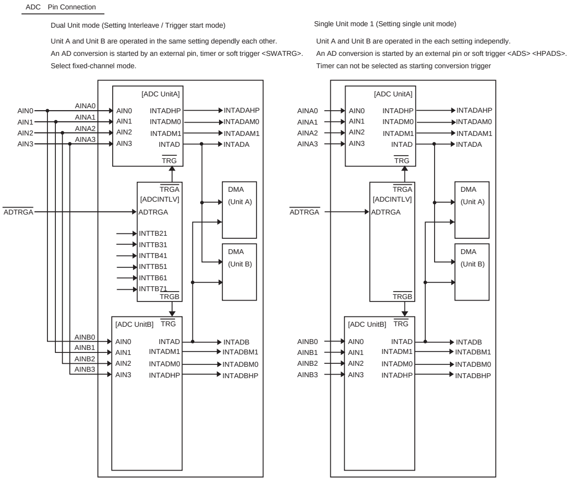
Figure 20-1 AD Converter Block Diagram
