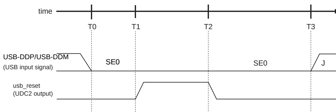
Figure 18-27 Reset Operation Timing
