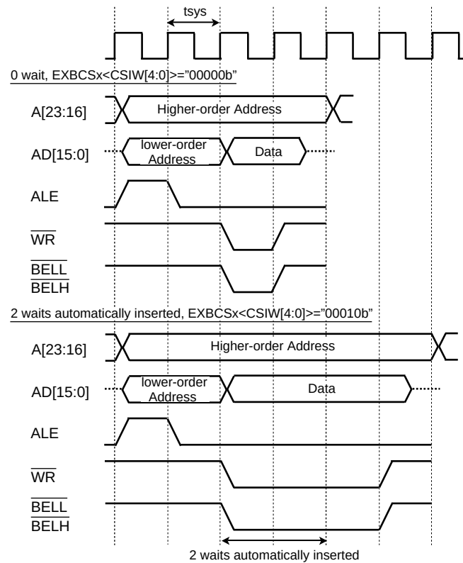
Figure 11-4 Write Operation Timing
