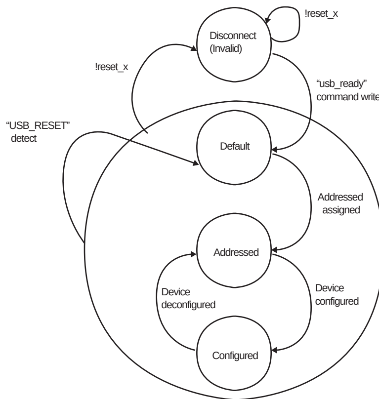
Figure 18-21 Device state diagram
