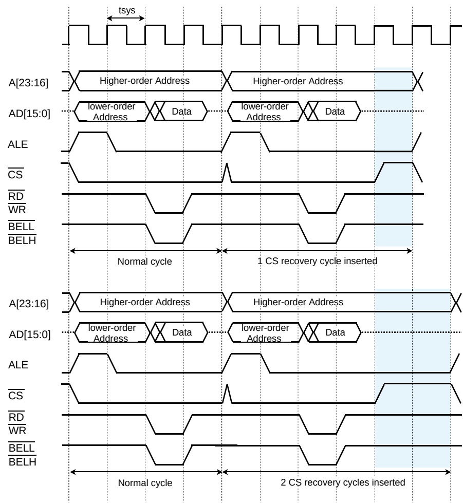
Figure 11-8 Timing of CS Recovery Time Insertion (ALE width: 1 clock)
