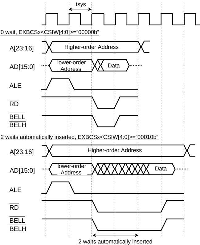
Figure 11-3 Read Operation Timing
