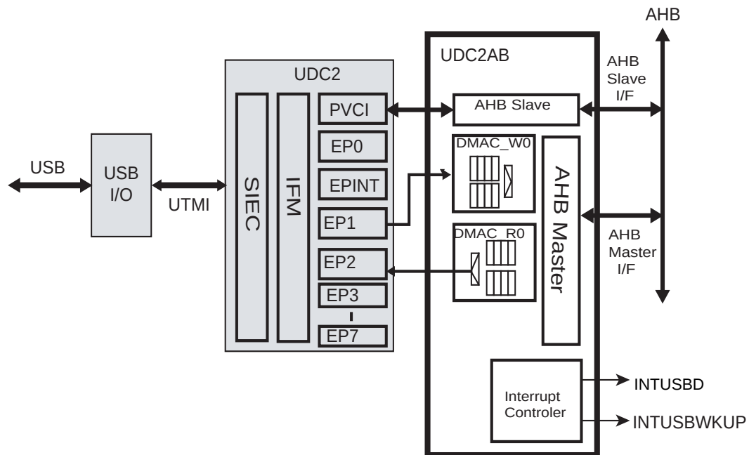
Figure 18-2 UDC2AB Block Diagram
