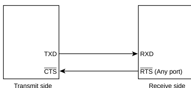
Figure 13-8 Handshake Function
