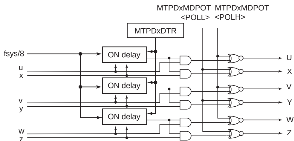
Figure 22-26 Schematic diagram of dead time circuit
