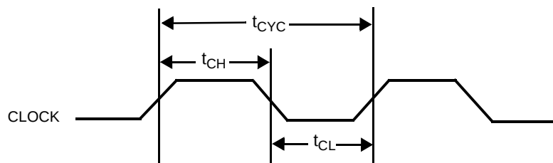
Figure 23-1. Clock Timing
