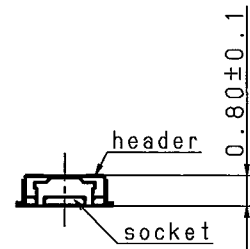
Setting drawing
