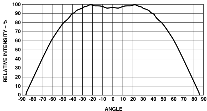
Figure 5b. Relative intensity vs. angle for HSMx-C177 and HSMx-C197.
