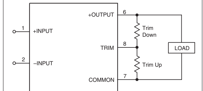
Figure 2b. Trim Connections Using Fixed Resistors
