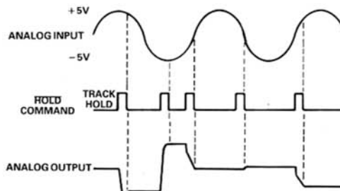
Figure 3. Sample/Hold Operation
