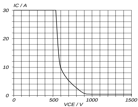
Fig.15. Reverse bias safe operating area. T_j \leq T_{j\text{max}}
