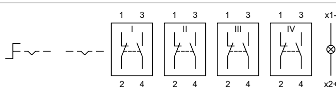
Wiring diagram 28
