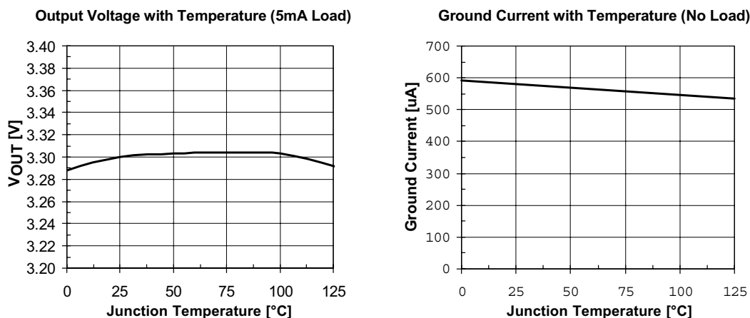
Figure 4. CM3002-33SA/SF & CM3002-33MA/MF Performance vs. Temperature
