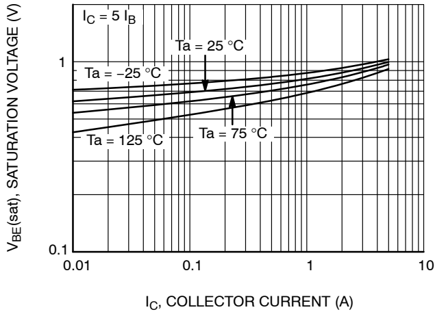
Figure 3. Saturation Voltage
