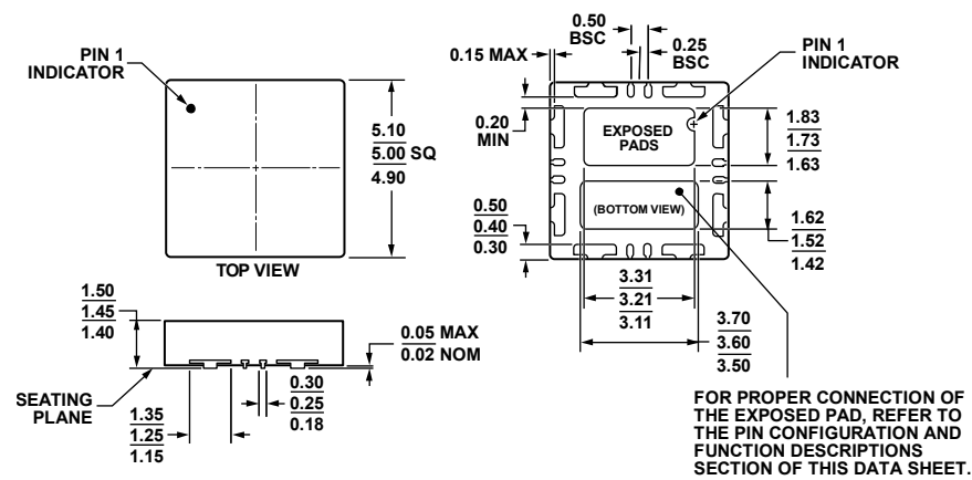
Figure 45. 16-Lead Lead Frame Chip Scale Package [LFCSP_LQ] 5 mm × 5 mm Body, Thick Quad (CP-16-8) Dimensions shown in millimeters
