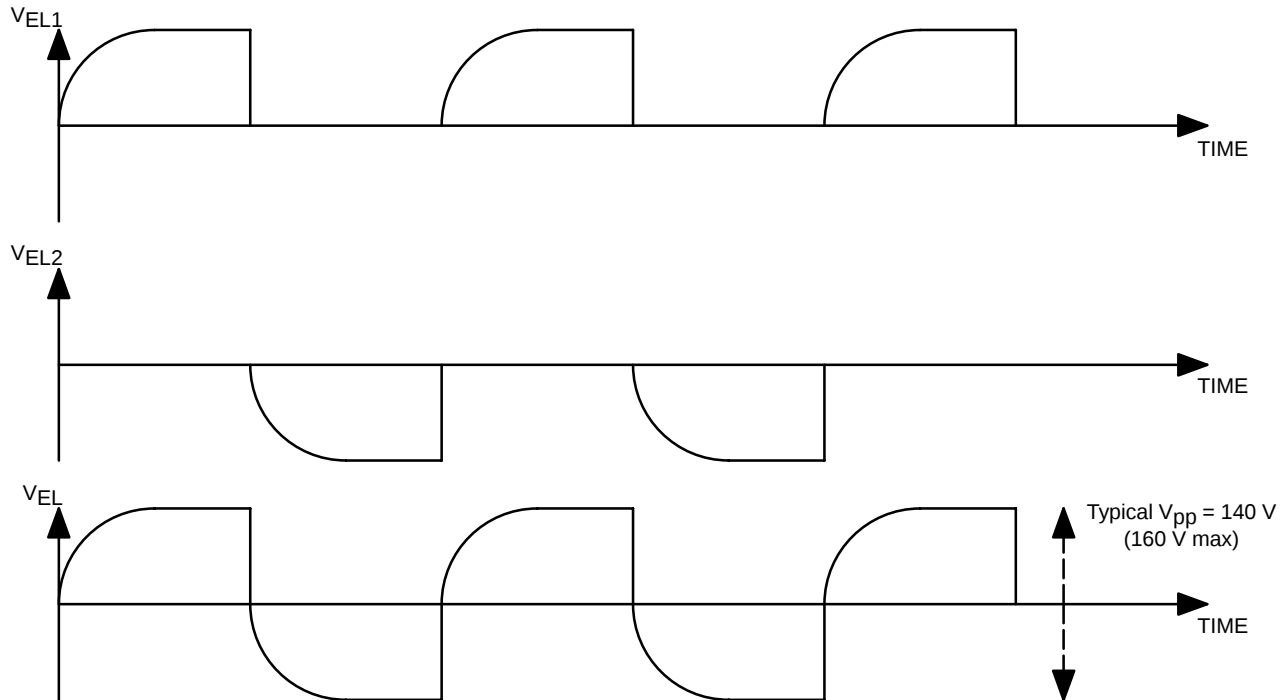
Figure 2. Output Waveform
