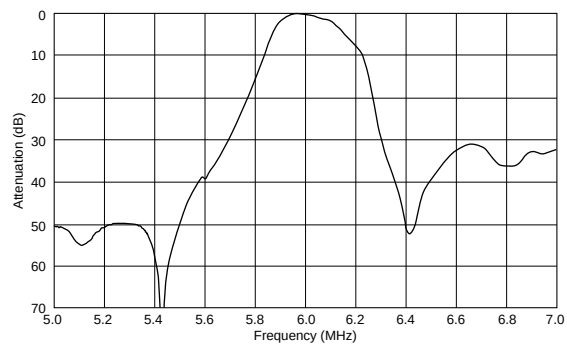
SFSRA6M00CF00-B0
