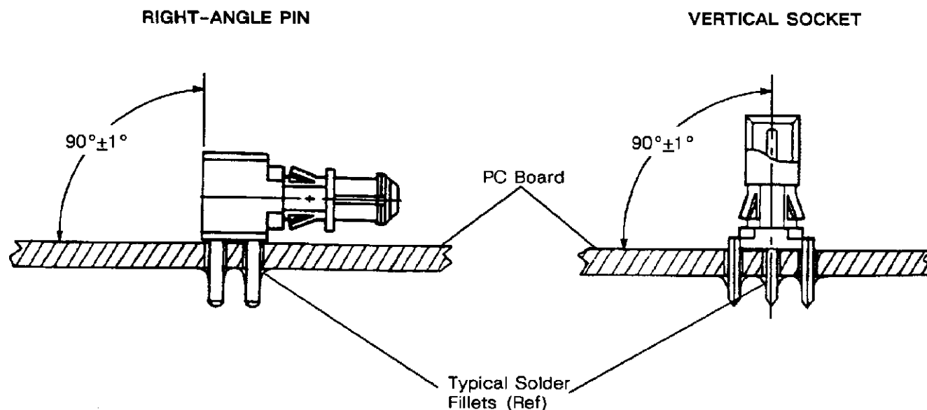
Fig. 3. Seated Contact Requirements
