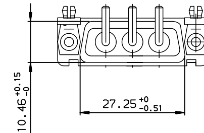
LAYOUT DIMENSIONS (after plating) CONNECTOR SIDE VIEW
