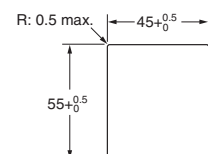
Mounting Hole Dimensions
