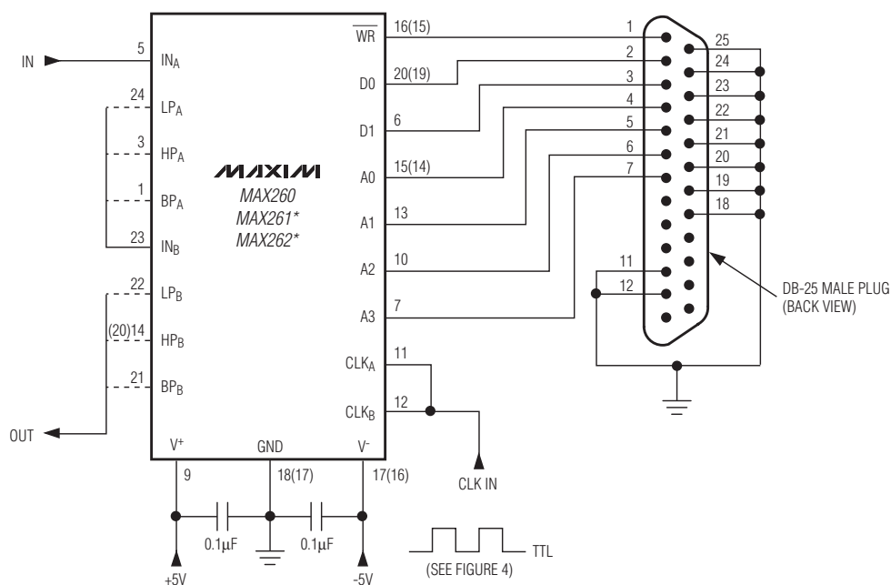
Figure 2. Basic Program and Hardware Connections to Parallel Printer Port for “Quick Look” Using a PC
