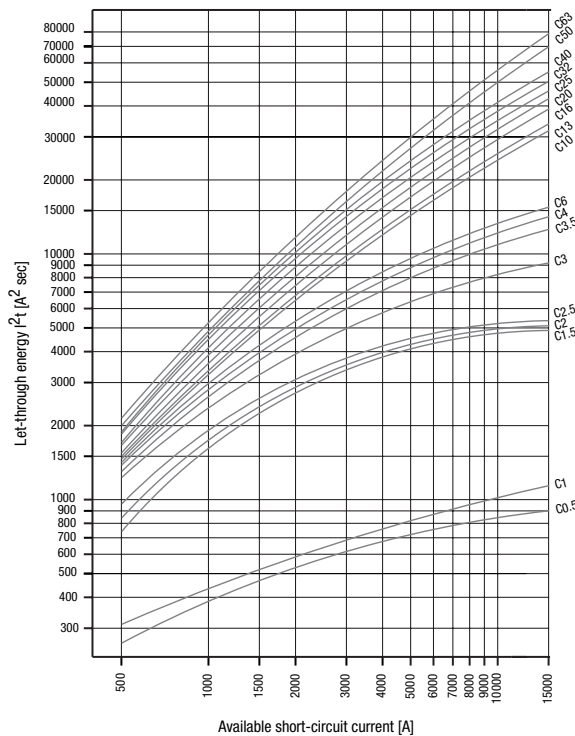
Maximum let-through energy L8 Type C
