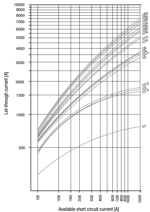
Maximum let-through current L8 Type C
