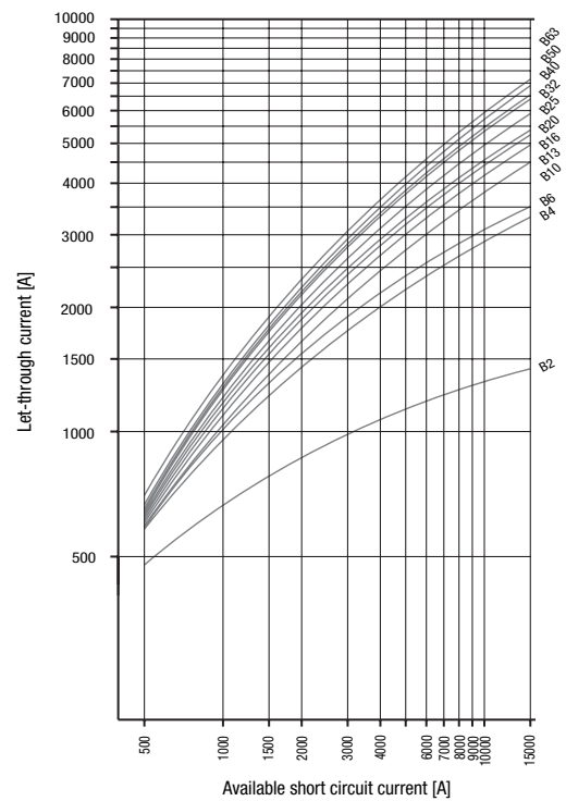
Maximum let-through current L8 Type B
