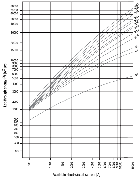
Maximum let-through energy L8 Type B
