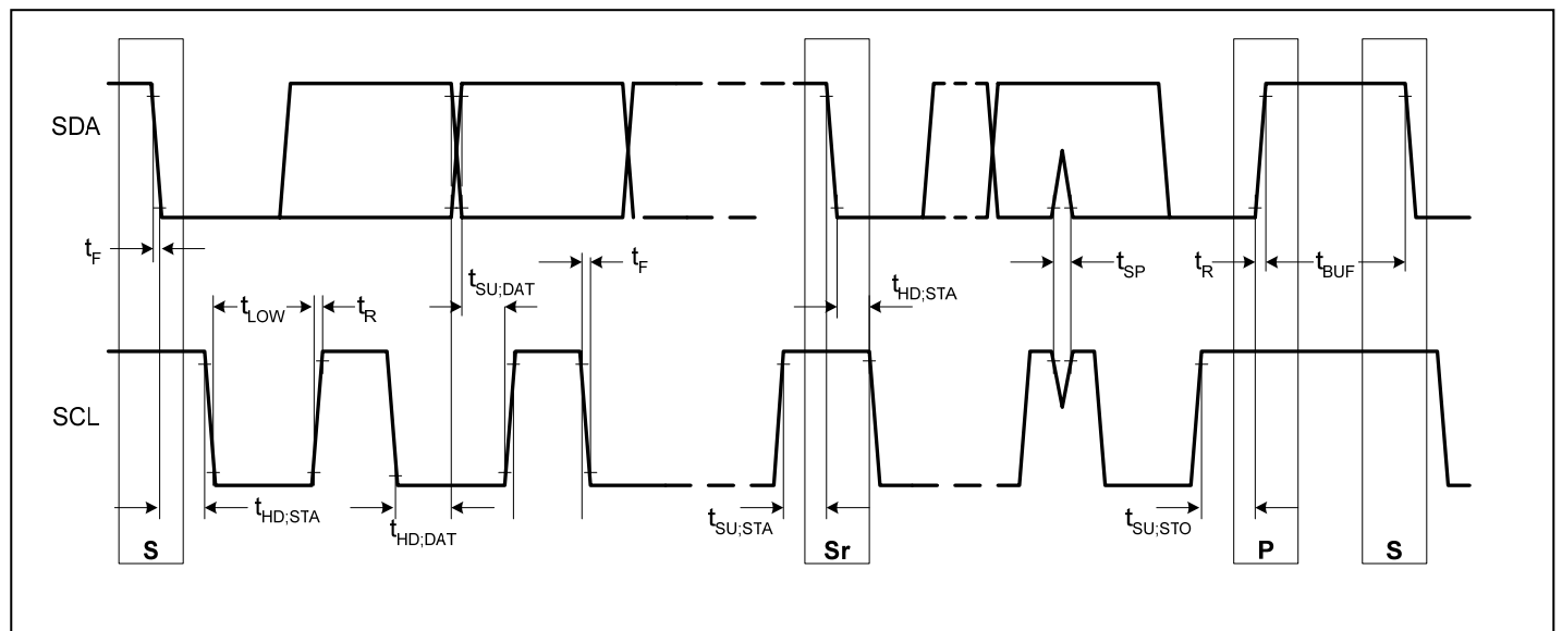
Figure 2. Timing Diagram
