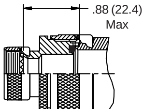
STYLE 2 (STRAIGHT See Note 1)
