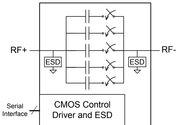
Figure 1. Functional Diagram
