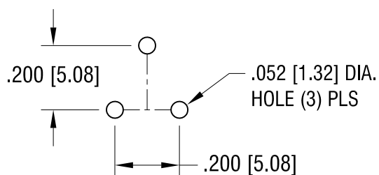
MOUNTING DETAIL
