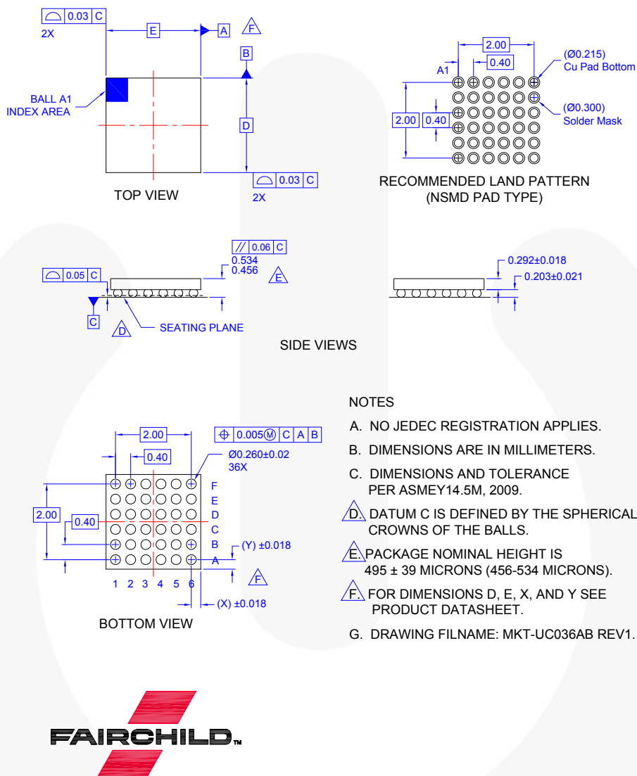
Figure 4. 36-Ball WLCSP, Non-JEDEC 2.415 mm x 2.415 mm, 0.4 mm Pitch
