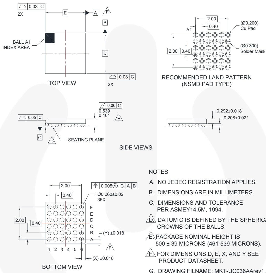
Figure 5. 36-Ball WLCSP, Non-JEDEC 2.36 mm x 2.36 mm, 0.4 mm Pitch
