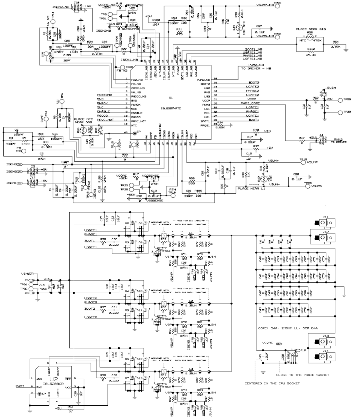
FIGURE 31. PORTION OF ISL6267EVAL1Z EVALUATION BOARD SCHEMATIC
