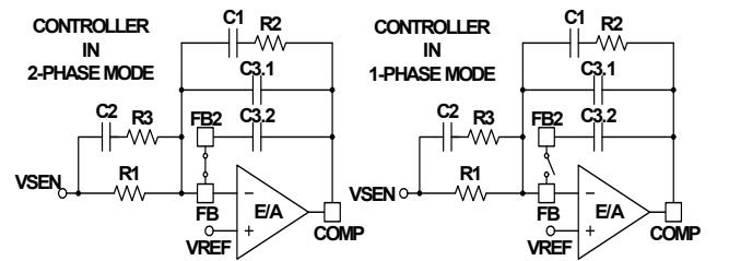
FIGURE 19. FB2 FUNCTION
