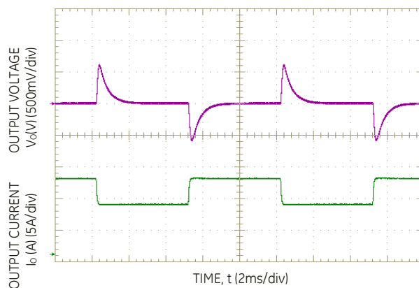
Figure 6. Dynamic Load Change Transient Response from 50 % to 75% to 50% of Full Load at Room Temperature and 48 Vin; 0.1A/uS, C_{o,ext} = 440\mu\text{F} .
