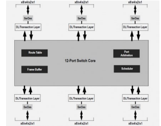
89H48H12G2 - Block Diagram
