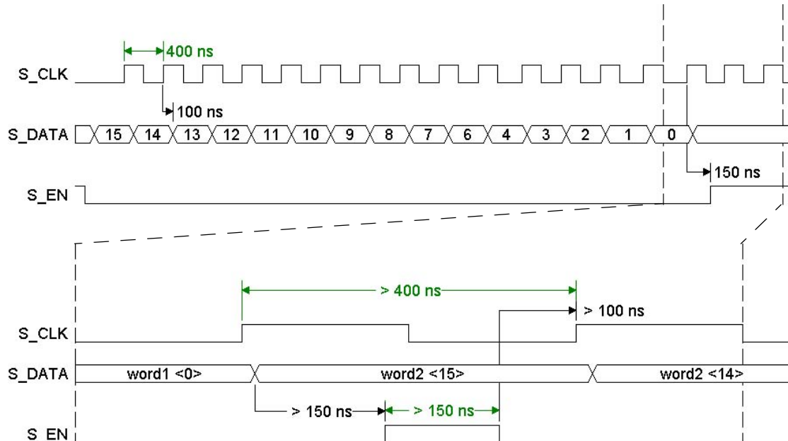
Figure 17. Serial-3-wire Interface Timing
