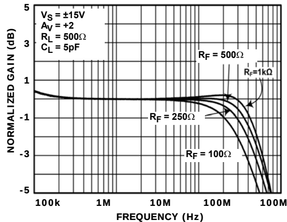
FIGURE 12. GAIN vs FREQUENCY FOR VARIOUS R_{FEEDBACK} ( A_V = +2 )
