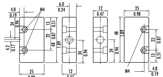
Switch - Type 1
