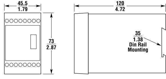
Control Unit 2
