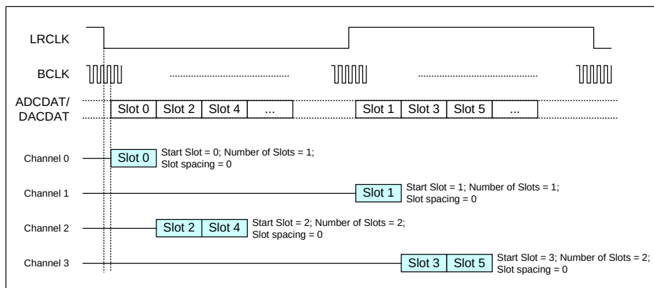
Figure 38 I2S Example
