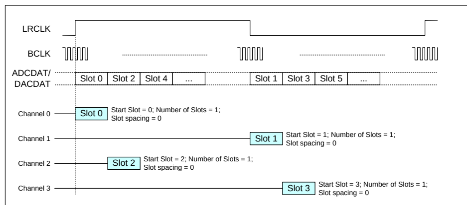
Figure 39 Left Justified Example
