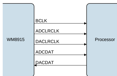
Figure 30 Master Mode
