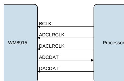
Figure 31 Slave Mode
