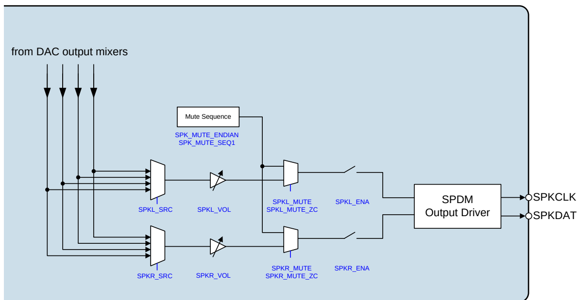
Figure 25 Digital Speaker Output (SPDM) Signal Paths
