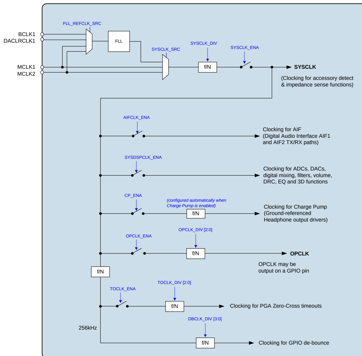
Figure 44 Clocking Scheme
