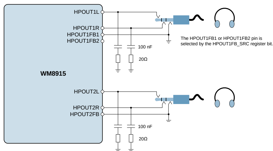
Figure 59 Headphone Connection
