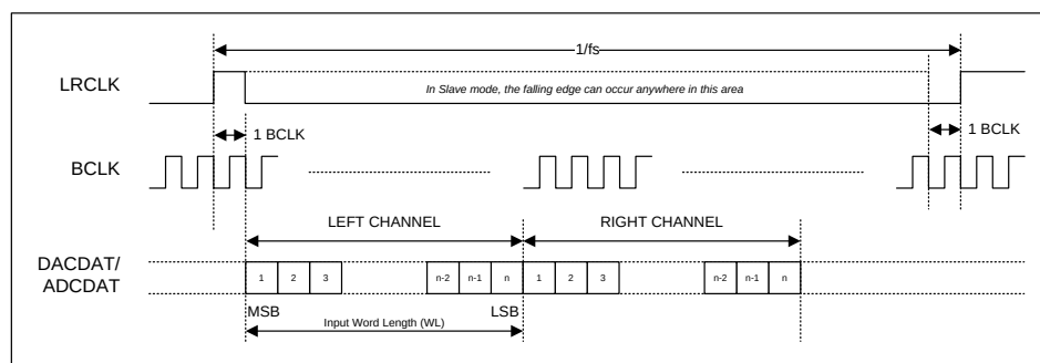
Figure 32 DSP Mode A Data Format
