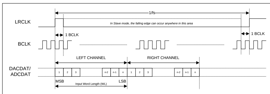
Figure 33 DSP Mode B Data Format
