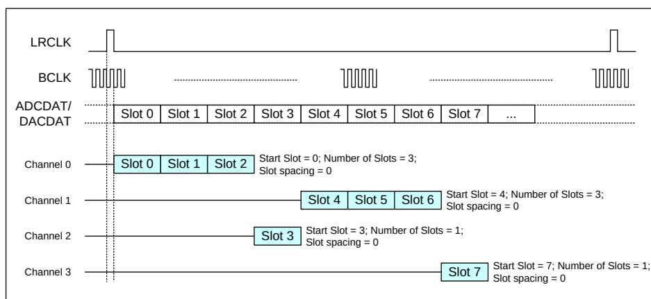
Figure 36 DSP Mode A Example
