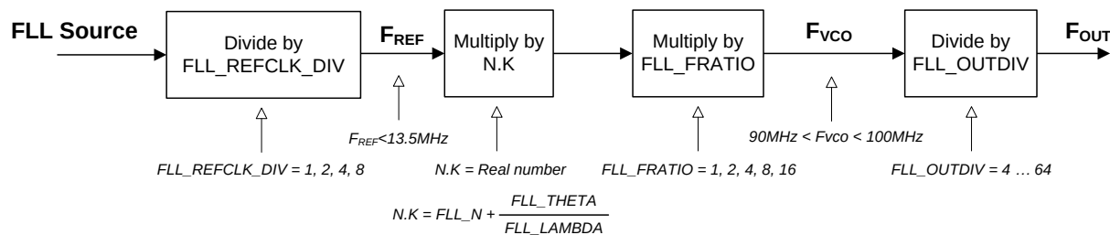
Figure 46 FLL Configuration
