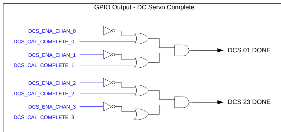
Figure 29 DC Servo Complete Status Output
