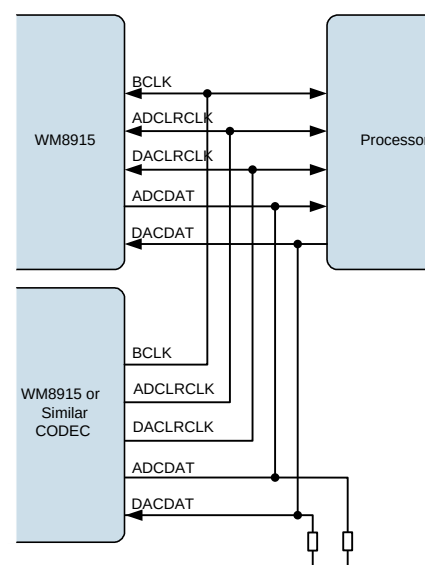
Figure 41 TDM with Other CODEC as Master
