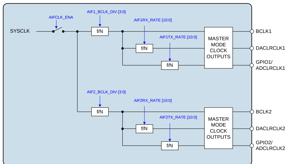
Figure 45 BCLK and LRCLK Control
