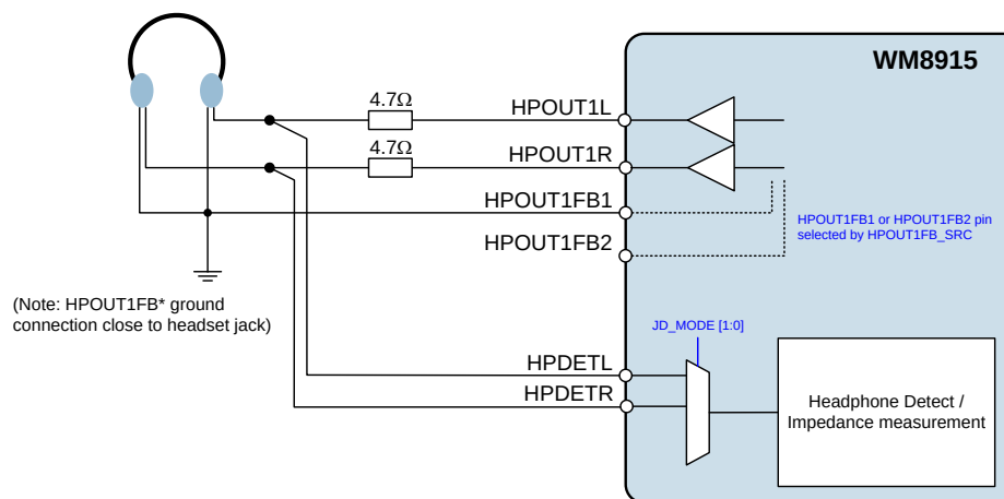
Figure 26 Headphone Detect Interface
