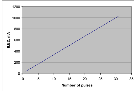
DAC linearity at V_{LED} = 500\text{mV}
