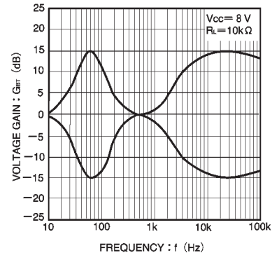
Fig. 5 Output gain vs. frequency
