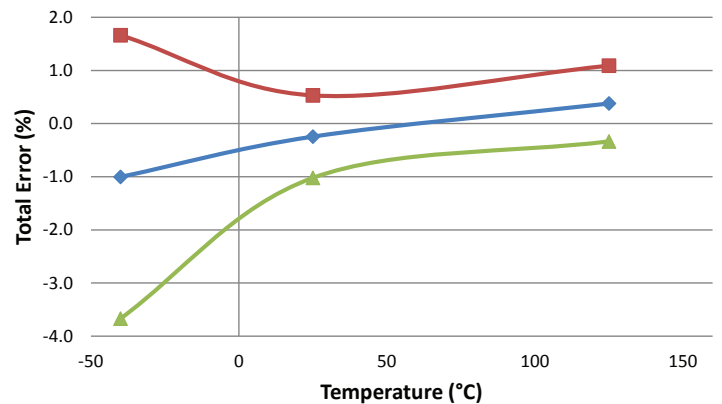
Total Error at I_{PR}(\text{max}) vs. Temperature
