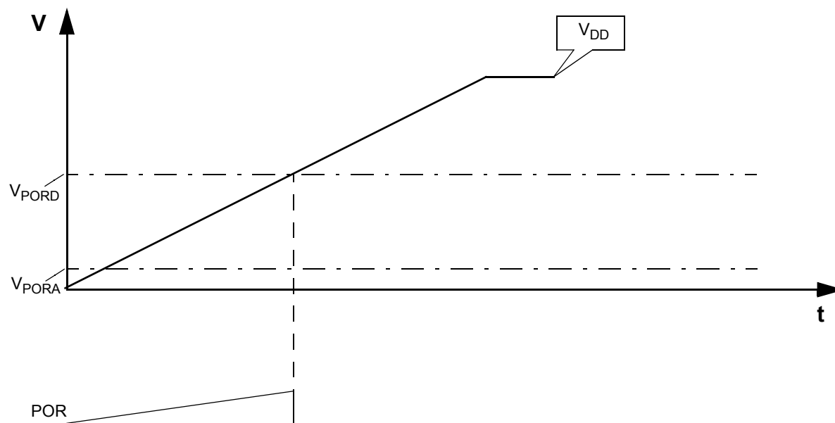
Figure 11. Power on Reset
