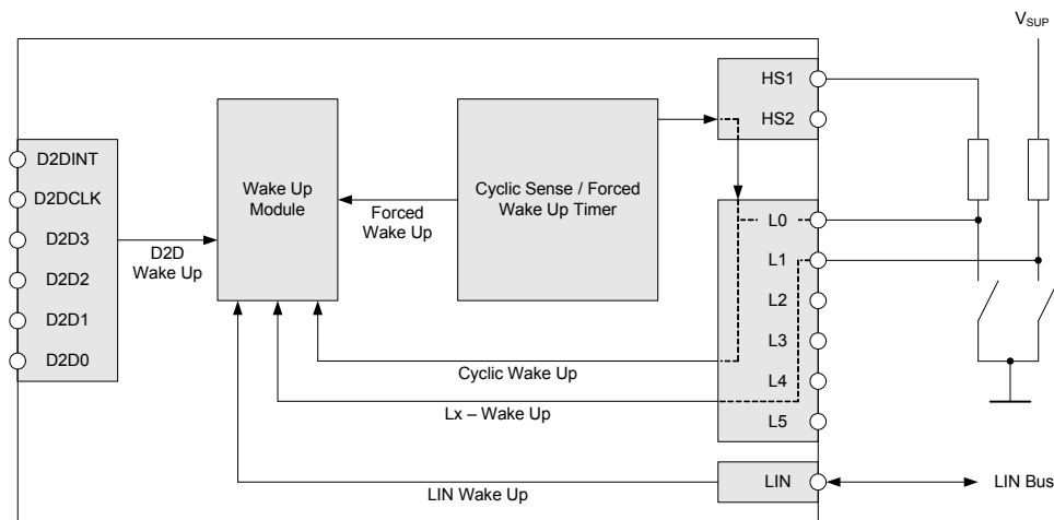
Figure 20. Wake-up Sources
