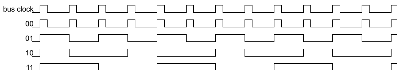
Figure 95. Interface Clock Waveforms for Various D2DCLKDIV Encoding
