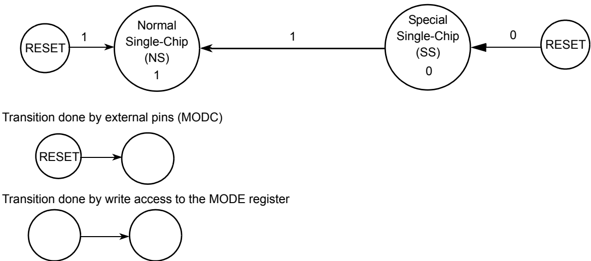
Figure 51. Mode Transition Diagram when MCU is Unsecured
