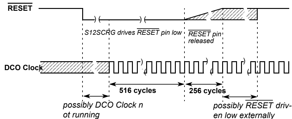
Figure 77. \overline{\text{RESET}} Timing
