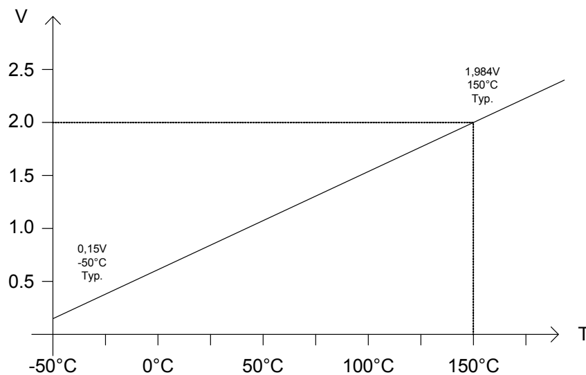
Figure 40. TSENSE - Graph
