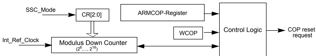
Figure 82. Block Diagram
