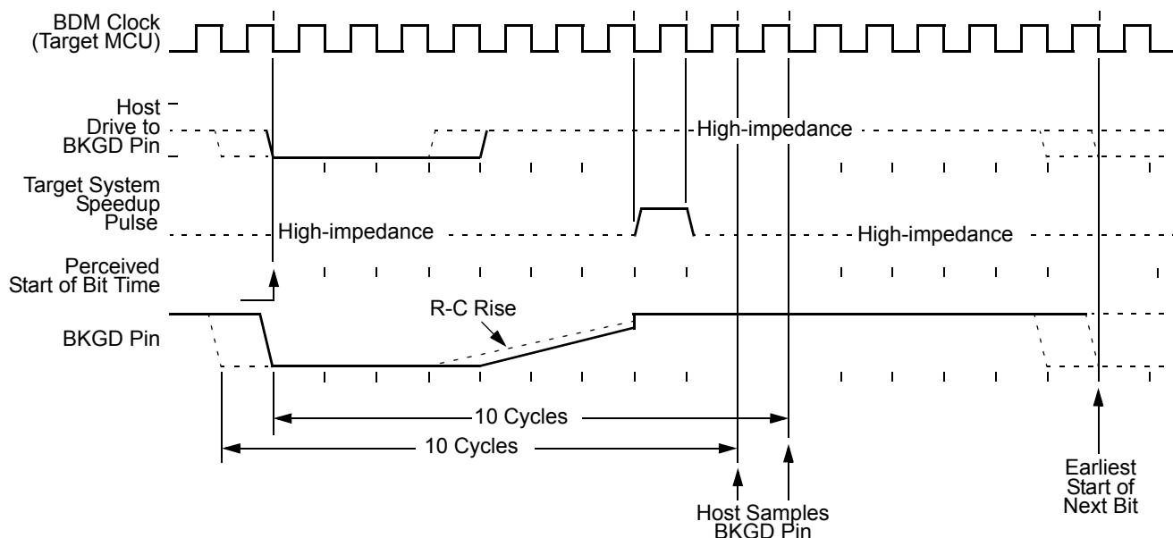
Figure 63. BDM Target-to-Host Serial Bit Timing (Logic 1)
