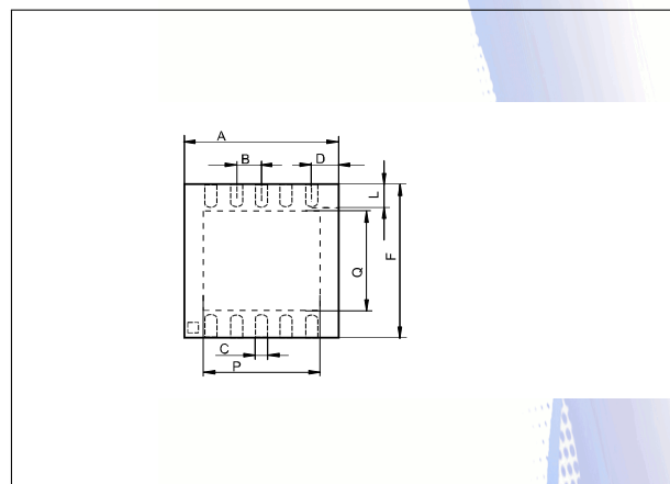
Figure 13.4: DFN-10 Package Dimensions.
