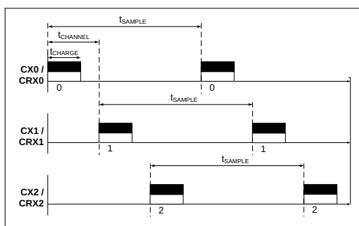
Figure 7.1: Boost power as on CX / CRx.
