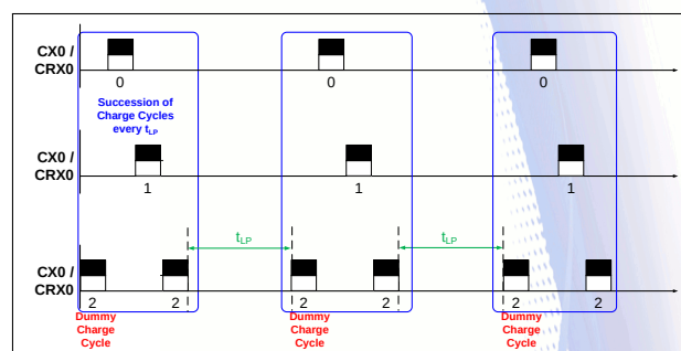
Figure 7.2: Charge cycles as charged in LP modes.
