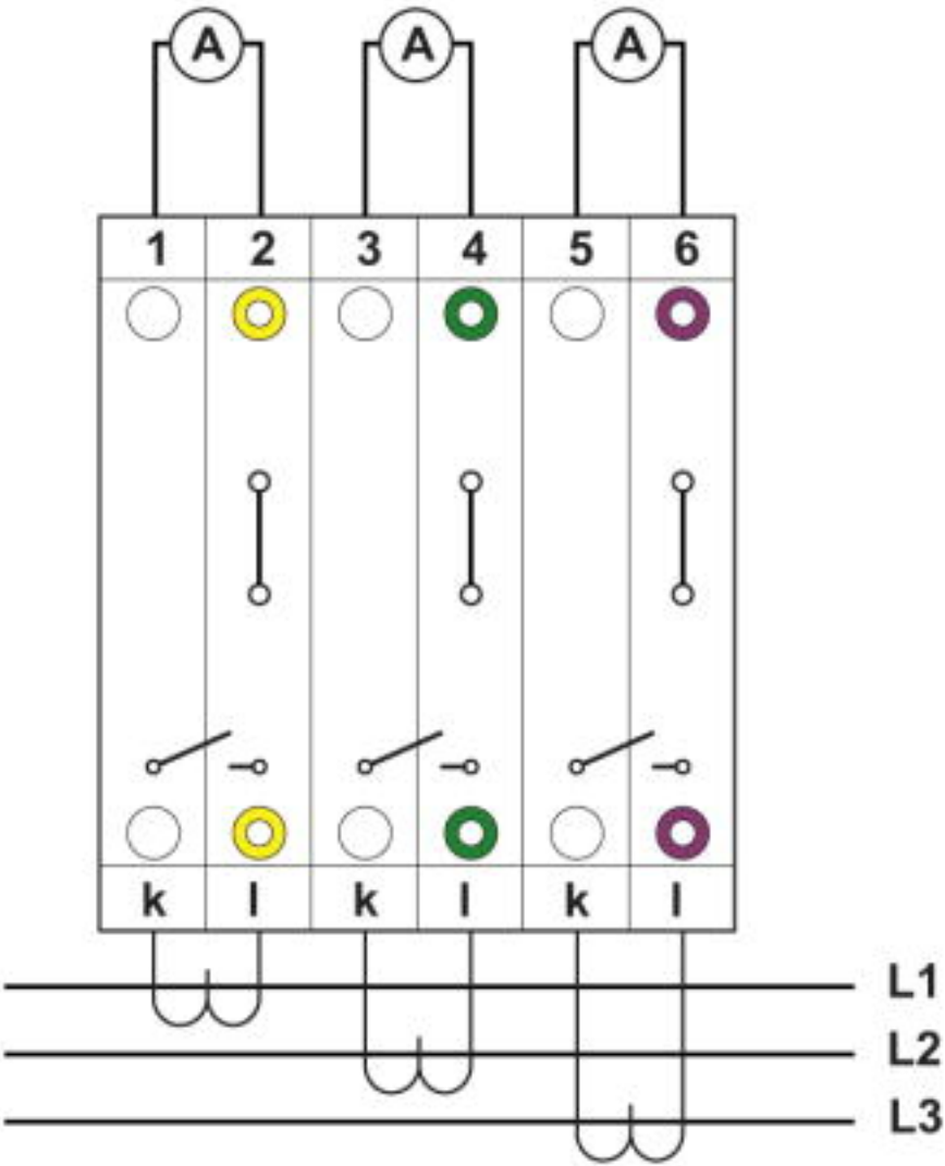
Connection diagram
