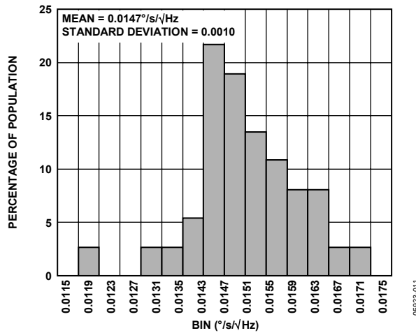
Figure 11. Noise Histogram
