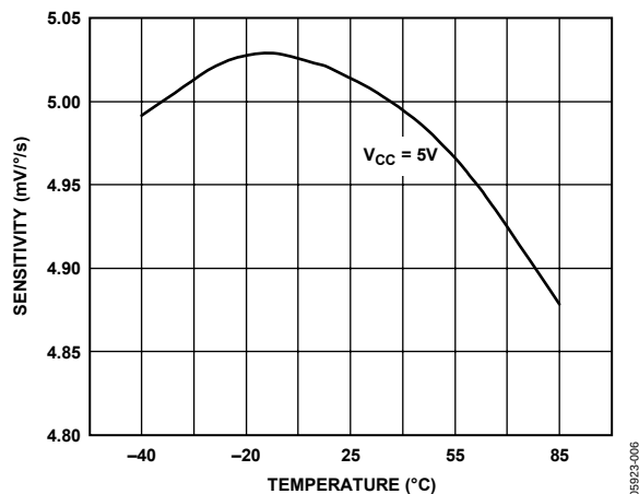
Figure 6. Gain Sensitivity vs. Temperature @ 300^{\circ}/s
