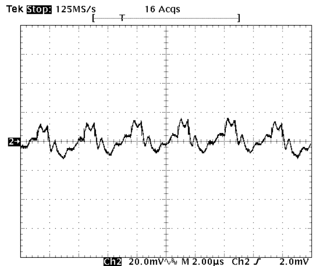
Fig-2.5V-5: Output voltage ripple (20mV/div.) for V_{out}=2.5V at full rated load current into a resistive load with external capacitance 47uF \times 4 ceramic + 1uF ceramic at V_{in}=12V .
