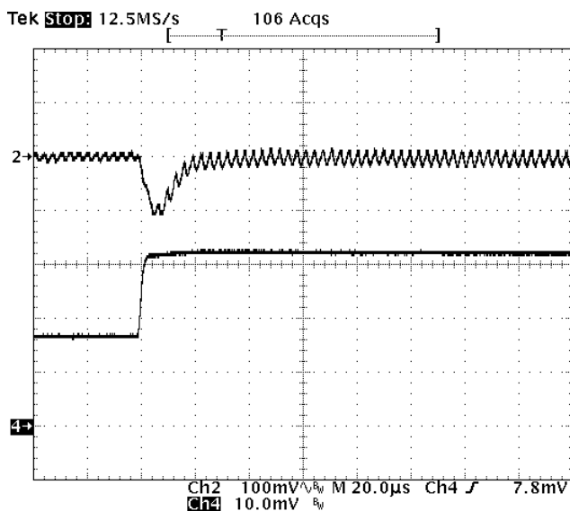
Fig-3.3V-6: Output voltage response for V_{out}=3.3V to positive load current step-change from 8A to 16A with slew rate of 5A/us at V_{in}=12V . C_o=47uF \times 4 ceramic.
