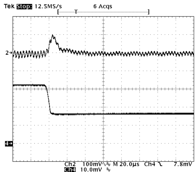
Fig-5.0V-7: Output voltage response for V_{out}=5.0V to negative load current step change from 16A to 8A with slew rate of -5A/us at V_{in}=12V . C_o=47uF \times 4 ceramic.
