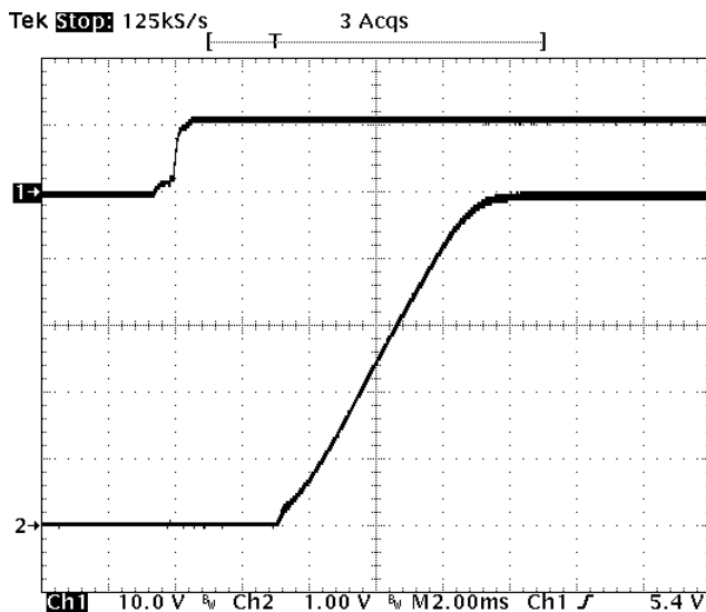
Fig-5.0V-4: Turn-on transient for V_{out}=5.0V with application of V_{in} at full rated load current (resistive) and 47uF \times 4 external capacitance at V_{in}=12V .
