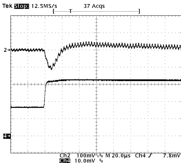
Fig-2.5V-6: Output voltage response for V_{out}=2.5V to positive load current step change from 8A to 16A with slew rate of 5A/us at V_{in}=12V . C_o=47uF \times 4 ceramic.
