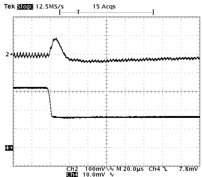
Fig-2.5V-7: Output voltage response for V_{out}=2.5V to negative load current step change from 16A to 8A with slew rate of -5A/us at V_{in}=12V . C_o=47uF \times 4 ceramic.
