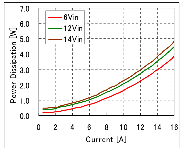
Fig-1.8V-3: Power Loss vs. load current and input voltage for V_{out}=1.8V . Airflow rate=200 LFM (1.0 m/s) and T_a=25^{\circ}C .
