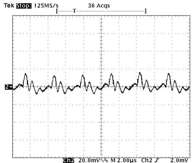
Fig-1.5V-5: Output voltage ripple (20mV/div.) for V_{out}=1.5V at full rated load current into a resistive load with external capacitance 47uFx4 ceramic + 1uF ceramic at V_{in}=12V .
