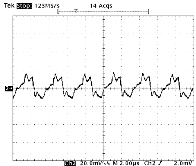
Fig-3.3V-5: Output voltage ripple (20mV/div.) for V_{out}=3.3V at full rated load current into a resistive load with external capacitance 47uF \times 4 ceramic + 1uF ceramic at V_{in}=12V .
