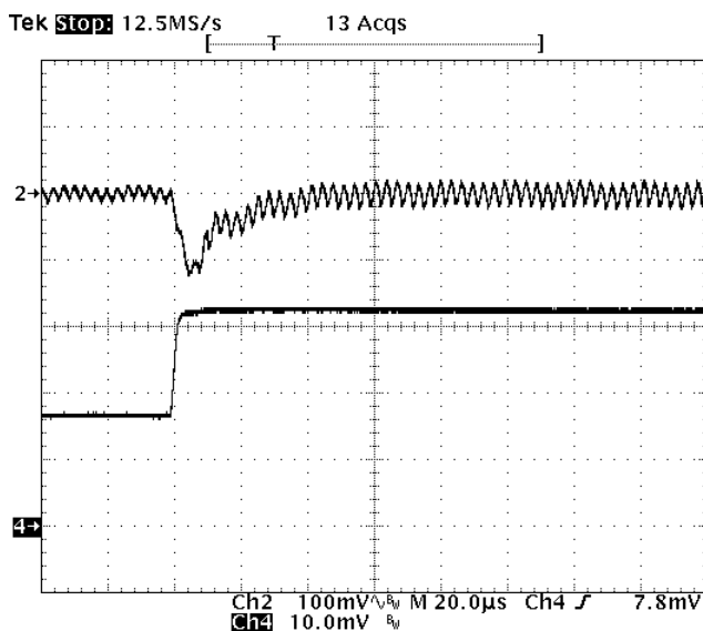
Fig-5.0V-6: Output voltage response for V_{out}=5.0V to positive load current step change from 8A to 16A with slew rate of 5A/us at V_{in}=12V . C_o=47uF \times 4 ceramic.
