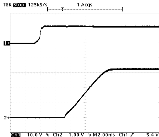
Fig-3.3V-4: Turn-on transient for V_{out}=3.3V with application of V_{in} at full rated load current (resistive) and 47uF \times 4 external capacitance at V_{in}=12V .
