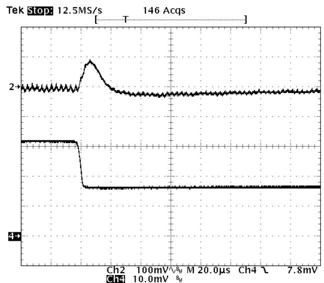
Fig-1.8V-7: Output voltage response for V_{out}=1.8V to negative load current step change from 16A to 8A with slew rate of -5A/us at V_{in}=12V . C_o=47uFx4 ceramic.
