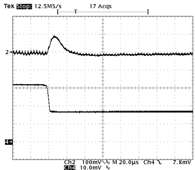
Fig-1.5V-7: Output voltage response for V_{out}=1.5V to negative load current step change from 16A to 8A with slew rate of -5A/us at V_{in}=12V . C_o=47uFx4 ceramic.
