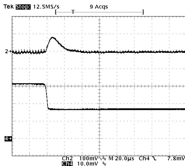
Fig-1.0V-7: Output voltage response for V_{out}=1.0V to negative load current step change from 16A to 8A with slew rate of -5A/us at V_{in}=12V . C_o=47uFx4 ceramic.
