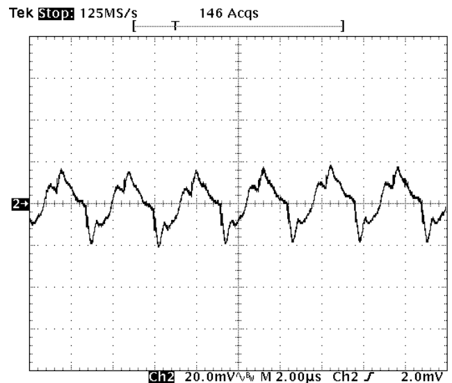
Fig-5.0V-5: Output voltage ripple (20mV/div.) for V_{out}=5.0V at full rated load current into a resistive load with external capacitance 47uF \times 4 ceramic + 1uF ceramic at V_{in}=12V .
