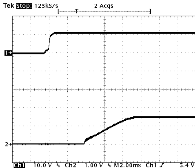
Fig-1.5V-4: Turn-on transient for V_{out}=1.5V with application of V_{in} at full rated load current (resistive) and 47uFx4 external capacitance at V_{in}=12V .
