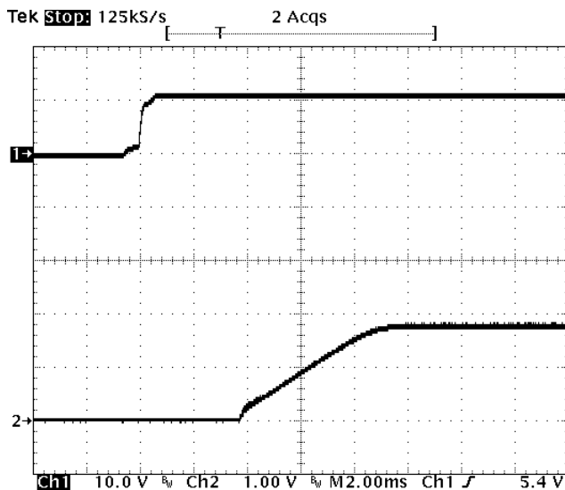
Fig-1.8V-4: Turn-on transient for V_{out}=1.8V with application of V_{in} at full rated load current (resistive) and 47uFx4 external capacitance at V_{in}=12V .
