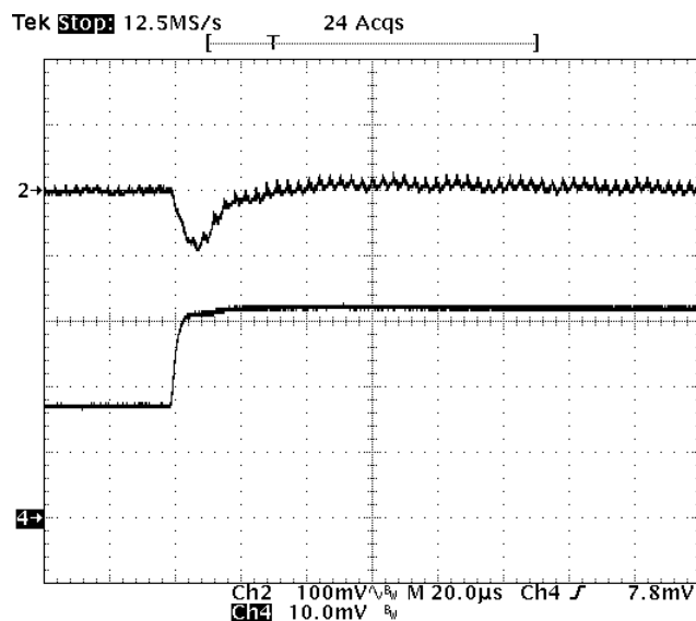
Fig-1.5V-6: Output voltage response for V_{out}=1.5V to positive load current step change from 8A to 16A with slew rate of 5A/us at V_{in}=12V . C_o=47uFx4 ceramic.
