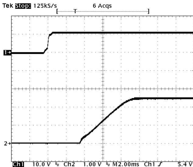
Fig-2.5V-4: Turn-on transient for V_{out}=2.5V with application of V_{in} at full rated load current (resistive) and 47uF \times 4 external capacitance at V_{in}=12V .
