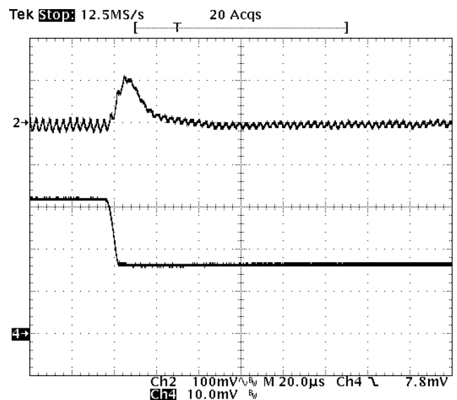
Fig-3.3V-7: Output voltage response for V_{out}=3.3V to negative load current step change from 16A to 8A with slew rate of -5A/us at V_{in}=12V . C_o=47uF \times 4 ceramic.
