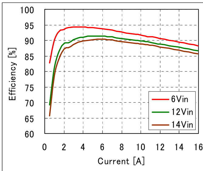
Fig-1.8V-2: Efficiency vs. load current and input voltage for V_{out}=1.8V . Airflow rate=200 LFM (1m/s) and T_a=25^{\circ}C .
