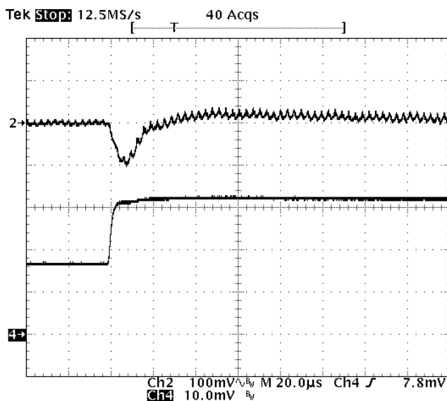
Fig-1.8V-6: Output voltage response for V_{out}=1.8V to positive load current step change from 8A to 16A with slew rate of 5A/us at V_{in}=12V . C_o=47uFx4 ceramic.
