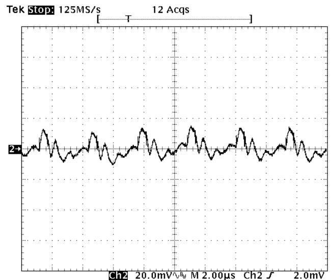
Fig-1.8V-5: Output voltage ripple (20mV/div.) for V_{out}=1.8V at full rated load current into a resistive load with external capacitance 47uFx4 ceramic + 1uF ceramic at V_{in}=12V .
