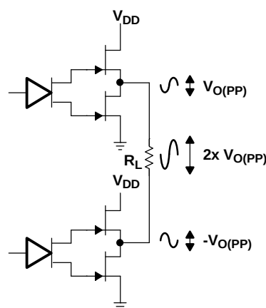
Figure 31. Differential Output Configuration
