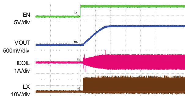
Fig. 11 - Start-Up, I_{OUT} = 0\text{ A} , Time = 1\text{ }\mu\text{s/div}
