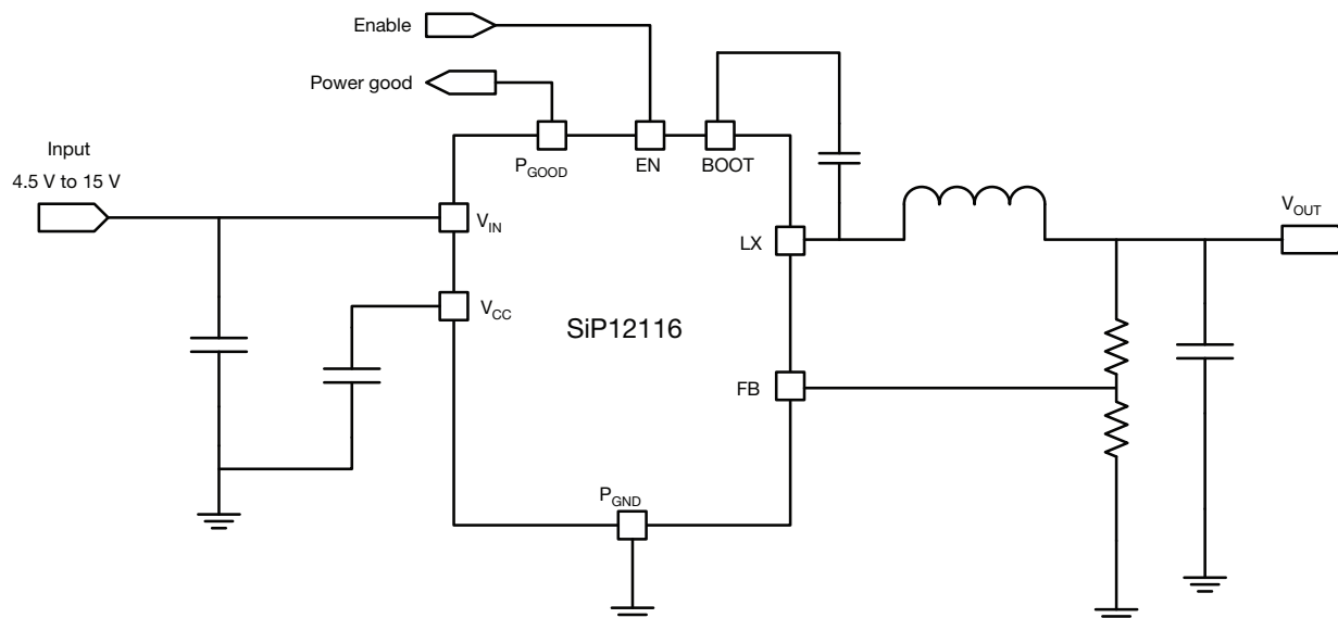
Fig. 1 - Typical Application Circuit for SiP12116
