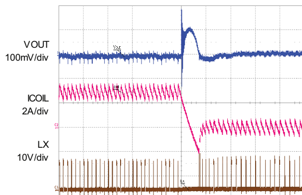
Fig. 13 - Load Step Overshoot Response, I_{OUT} = 3\text{ A} to 0\text{ A} , Time = 10\text{ }\mu\text{s/div}
