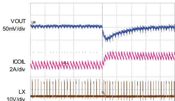
Fig. 9 - Load Step Undershoot Response, I_{OUT} = 0\text{ A} to 1.5\text{ A} , Time = 10\text{ }\mu\text{s/div}
