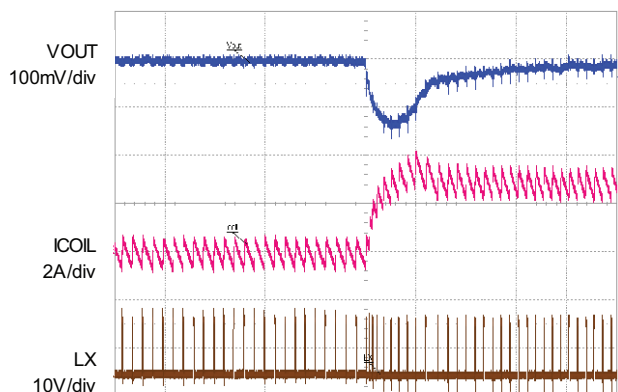
Fig. 10 - Load Step Undershoot Response, I_{OUT} = 0\text{ A} to 3\text{ A} , Time = 10\text{ }\mu\text{s/div}
