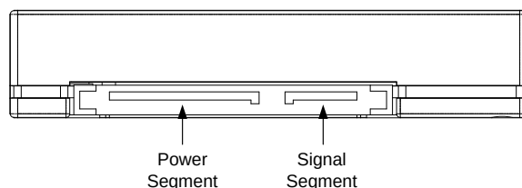
Figure 3: SSD Serial ATA 2.5" Pin Configuration
