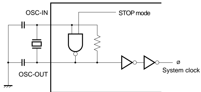
Figure 9-1. System Clock Generator
