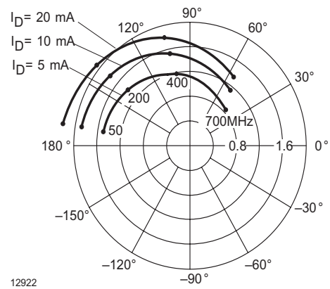
Figure 13. Forward Transmission Coefficient
