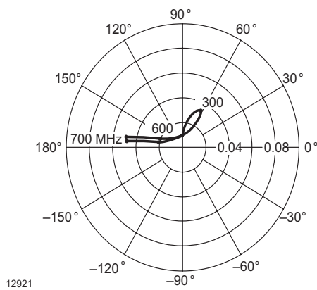
Figure 12. Reverse Transmission Coefficient
