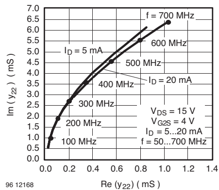
Figure 10. Short Circuit Output Admittance
