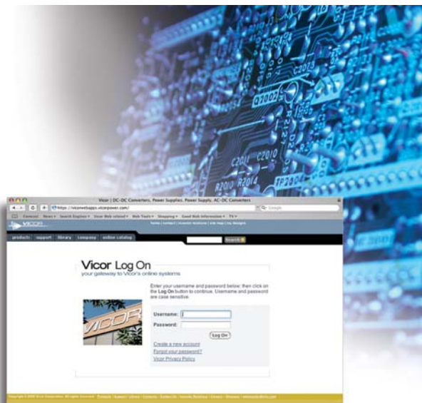
SINGLE SIGN-ON
