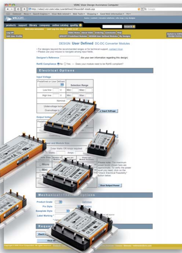
SINGLE SIGN-ON
