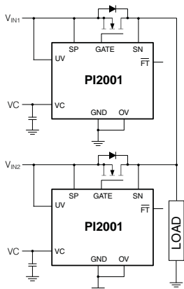
High-side Active ORing
