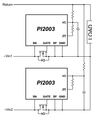
Low-side Active ORing
