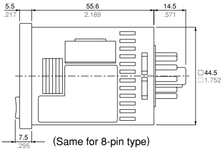
Pin type (embedded installation/ front panel installation)
