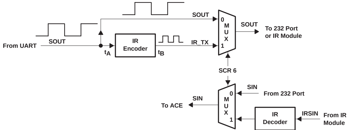
Figure 28. TL16PIR552 Mode Select
