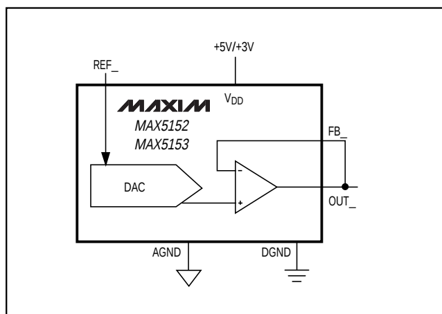
Figure 9. Unipolar Output Circuit
