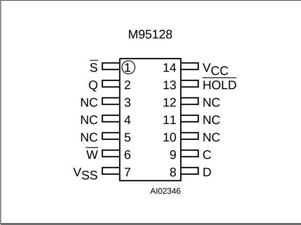
Figure 2C. TSSOP Connections
