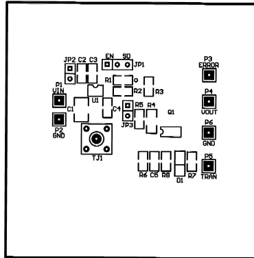
FIGURE 8. Silk Screen—Si9181
