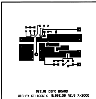
FIGURE 9. Top Layer—Si9181
