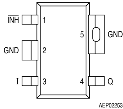
Figure 1 Pin Configuration (top view)
